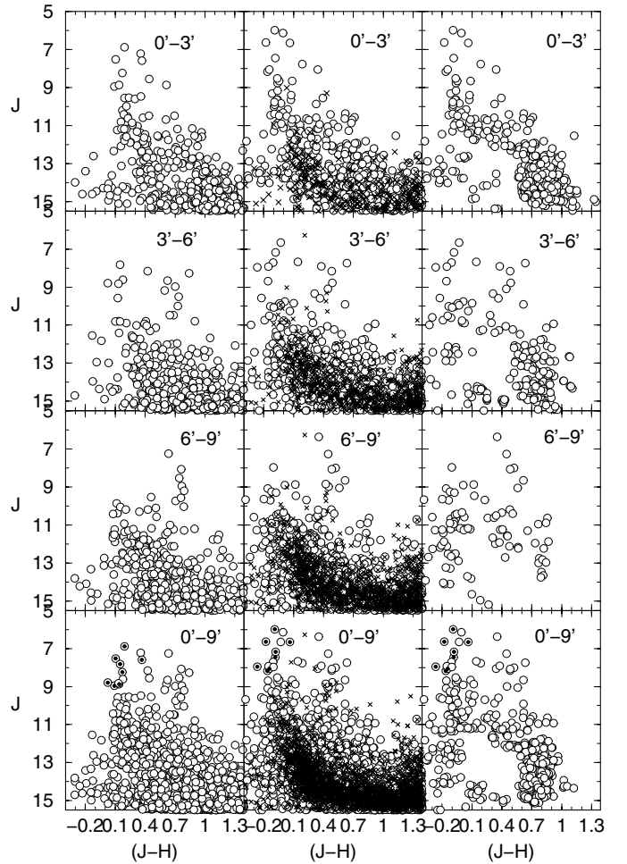
Fig. 3. J \times (J - H) CMDs of the central 9' of NGC 6611. Left panels: observed photometry. Middle panels: reddening-corrected CMDs according to Belikov et al. (1999). Right panels: reddening-corrected and field-star decontaminated CMDs. Note the extended MS and conspicuous PMS population, which is restricted essentially to the central 6' . Field stars are shown as x in the middle panels. Filled circles in the bottom panels: O V stars from Bosch et al. (1999).
