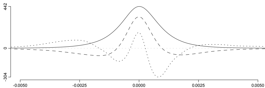
Figure 2.7: The estimated mean-function \hat{\mu} (solid), and the eigenfunctions \hat{\psi}_1 (dashed) and \hat{\psi}_2 (dotted). The eigenfunctions are rescaled by a 10\times factor for better visualization.
