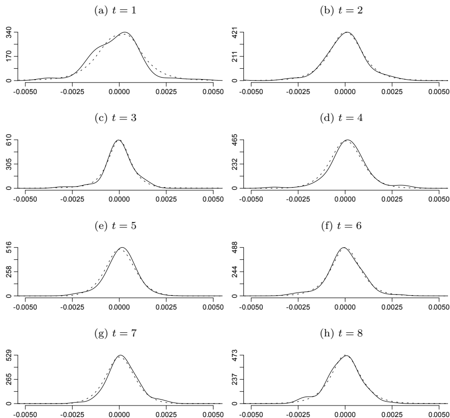
Figure 2.6: Non-parametric density estimates Y_t (solid) and filtered estimates \widehat{X}_t (dotted), t = 1, \dots, 8 .
