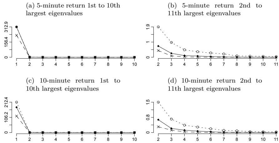
Figure 2.3: 5- and 10-minute return largest estimated eigenvalues using bandwidths \hat{h}_t (solid), 0.5\hat{h}_t (dotted) and 2\hat{h}_t (dashed).
