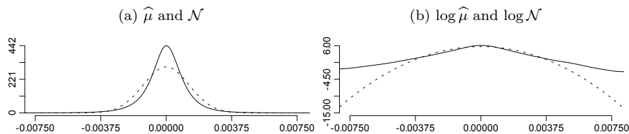
Figure 2.9: (A) The pdf \hat{\mu} (solid) and a Gaussian pdf \mathcal{N} of same mean and variance (dotted); (B) The corresponding log-pdf's.
