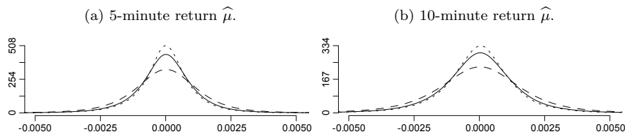
Figure 2.2: Estimated mean-function \hat{\mu} for the (A) 5- and (B) 10-minute return obtained using bandwidths \hat{h}_t (solid), 0.5\hat{h}_t (dotted) and 2\hat{h}_t (dashed).
