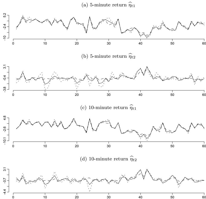
Figure 2.5: 5- and 10-minute return estimated loadings \hat{\eta}_{t1} and \hat{\eta}_{t2} for t = 1, \dots, 60 , using bandwidths \hat{h}_t (solid), 0.5\hat{h}_t (dotted) and 2\hat{h}_t (dashed).
