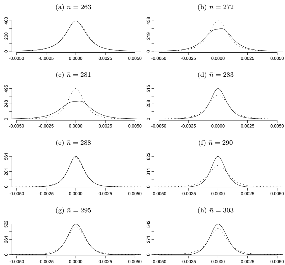
Figure 2.11: Pdf forecasts \tilde{X}_{\bar{n}|\bar{n}-1} (dotted) and realized filtered pdf's \hat{X}_{\bar{n}|\bar{n}} (solid); (A) \bar{n} = 263 , best prediction according to \nabla_{\bar{n}} ; (B) \bar{n} = 272 , selected at random; (C) \bar{n} = 281 , worst prediction according to both measures; (D) \bar{n} = 283 , closest-to-the-mean \Delta_{\bar{n}} ; (E) \bar{n} = 288 , best prediction according to \Delta_{\bar{n}} ; (F) \bar{n} = 290 , selected at random; (G) \bar{n} = 295 , selected at random; (H) \bar{n} = 303 , closest-to-the-mean \nabla_{\bar{n}} . See Table 2.5 for the values of \Delta_{\bar{n}} and \nabla_{\bar{n}} at those dates.
