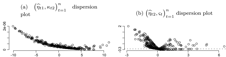
Figure 2.8: Dispersion plots of (A) \hat{\eta}_{t1} vs. \kappa_{t2} , and (B) \hat{\eta}_{t2} vs. \zeta_t . The dotted line in panel (B) indicates the vertical-axis's zero.
