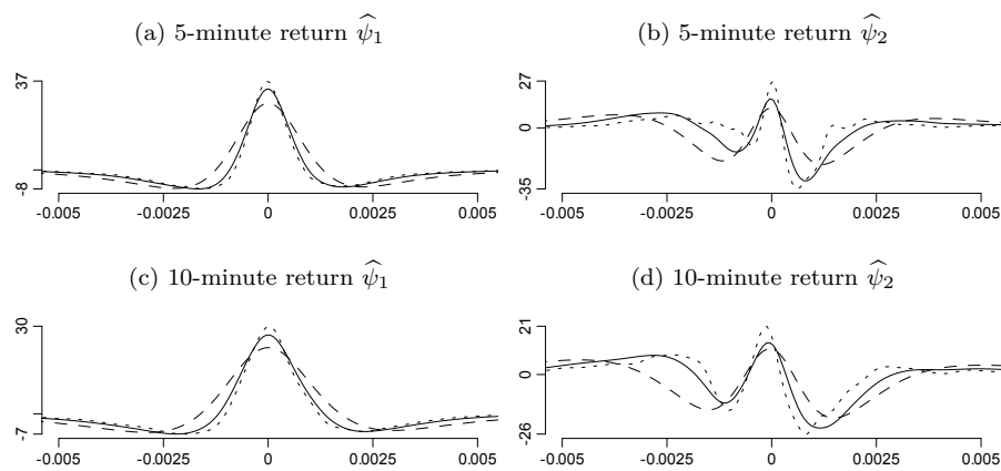
Figure 2.4: 5- and 10-minute return estimated eigenfunctions using bandwidths \hat{h}_t (solid), 0.5\hat{h}_t (dotted) and 2\hat{h}_t (dashed).
