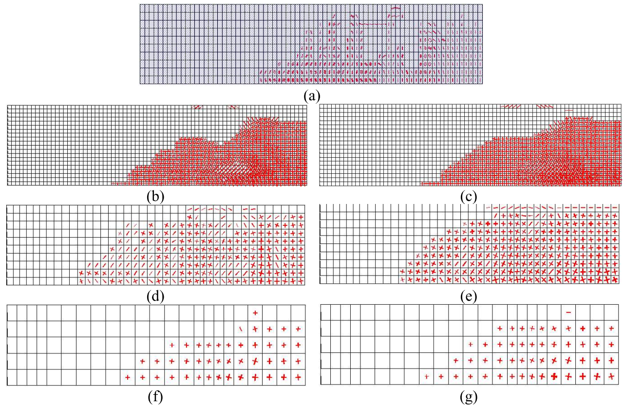
Figura 9 – Fissuras (a) S65_1_WW, (b) S186_1_C, (c) S186_1_B, (d) S186_2_C, (e) S186_2_B, (f) S186_4_C e (g) S186_4_B
