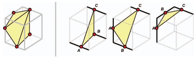
Fig. 2. The quality of each triangle generated by Marching Cubes depends on the combination of edges that generate the triangle.
