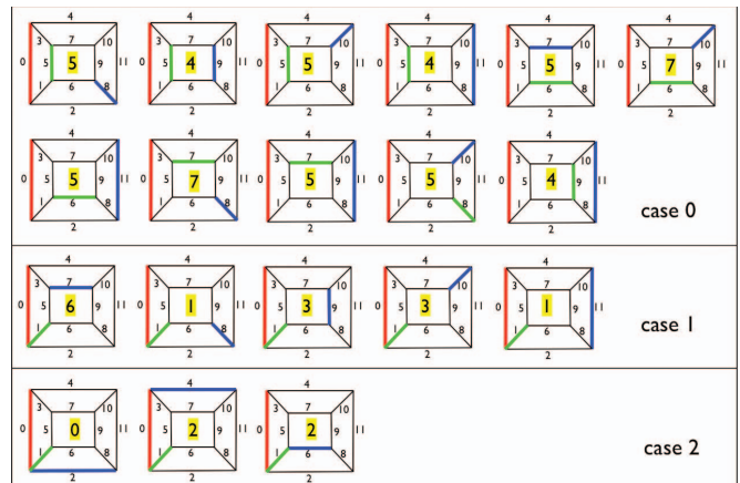
Fig. 9. Cases used to enumerate edge groups in a cubic cell.
