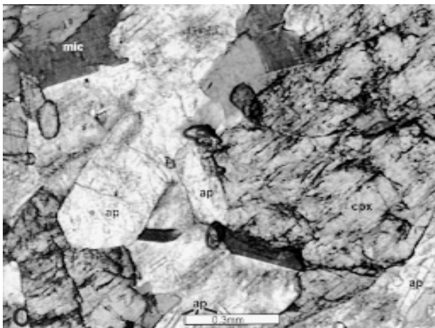
Figure 2 - Digital images obtained under light transmitted optical microscope. Anhedral late mica phenocryst including several aciculate apatites (A). Subhedral late mica phenocrysts enclosing poikilitically alkali feldspar and aciculate apatites, contrasting with the earlier crystallized euhedral grains. Note the straight contacts of euhedral crystals, and the sinuous contours of poikilitic phenocryst (B). Detail of euhedral early-crystallized apatite crystals (C).
