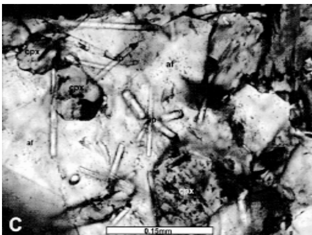
Figure 4 - Digital images obtained under light transmitted optical microscope. Aciculate apatite crystals enclosed poikilitically in alkali feldspar plates (A). Comparison between early-crystallized euhedral apatite, and aciculate grains originated during co-mingling (B). Detail of apatite needles included in alkali feldspar. It is also observed the occurrence of basal sections of elongate pyroxene crystals (C).
