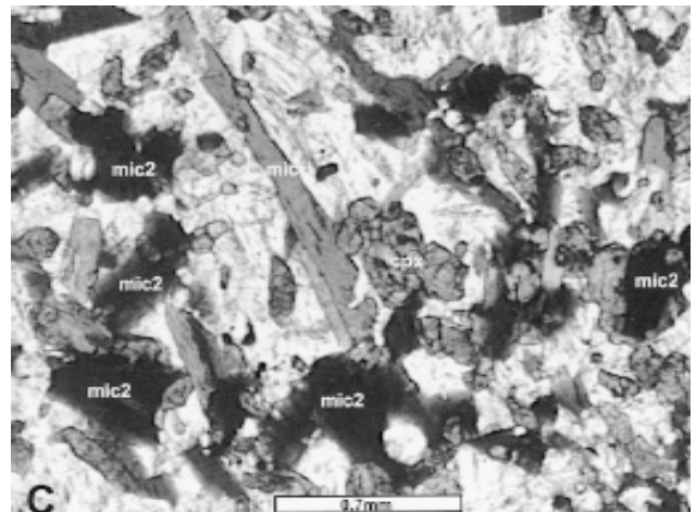
Figure 3 - Digital images obtained under light transmitted optical microscope. Elongate crystals of mica and pyroxene crystallized by quenching of hotter mafic magma against cooler felsic ones. The axial ratio of pyroxene is estimated around 12 (length:width), and slightly lower for mica crystals (A). Note the poikilitic character of alkali feldspar plates, corroborating its late-magmatic crystallization after co-mingling event (B). Two generations of groundmass mica crystals. Elongate grains crystallized during undercooling of mafic magma, and dark anhedral grains probably formed during a later magmatic stage (C).
