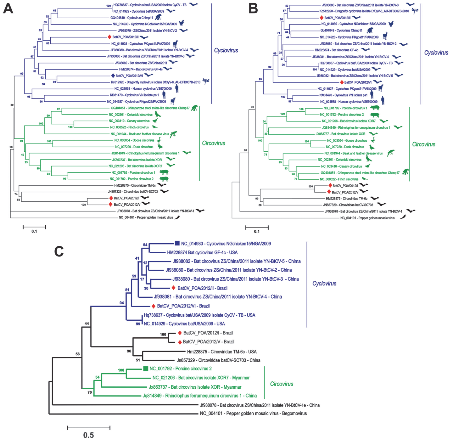
Fig 3. Phylogenetic analysis of the complete CAP (A), REP (B) and complete genomes (C) from Circovirus and Circovirus -like genomes identified in mammals, birds and insects. Host denomination is demonstrated after each retrieved sequence from GenBank with their accession numbers and clustered along, according to genus classification. The sequences identified in bat feces from Southern Brazil are labeled by red diamonds. Evolutionary analyses were conducted in MEGA5 [31].
