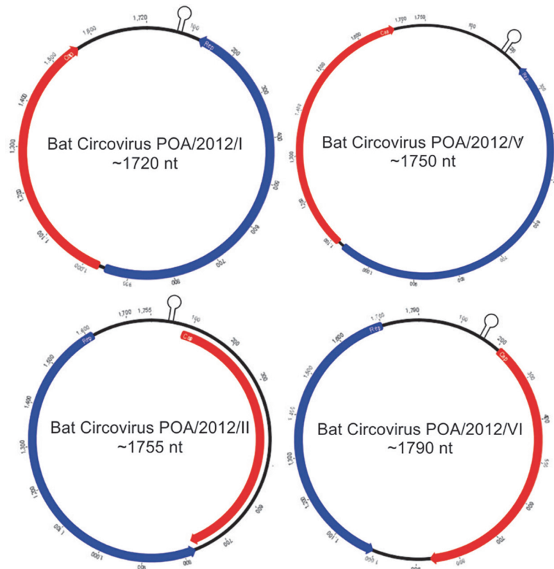
Fig 2. Predicted genome organization of the four circular ssDNA sequences with the locations of the potential stem-loop structures recovered from bat feces in Southern Brazil. The two inversely arranged ORFs responsible for encoding the putatives replication associated protein (REP) and capsid protein (CAP) are shown in blue and red boxes, respectively.
