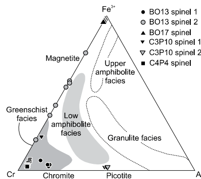
Figure 15. Chemical classification diagram of Cr-spinel from Bossoroca ophiolite. Compositional fields of metamorphosed spinel shown (modified from Abdel-Karim and El-Shafei 2018). Composition of minerals indicated.
