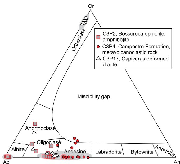
Figure 17. Chemical classification diagram of feldspar. Main
