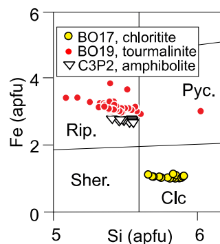
Rip.: ripidolite; Clc.: clinocllore; Pyc.: picnochlorite; Sher.: sheridinite. Source: based on Hey (1954)
