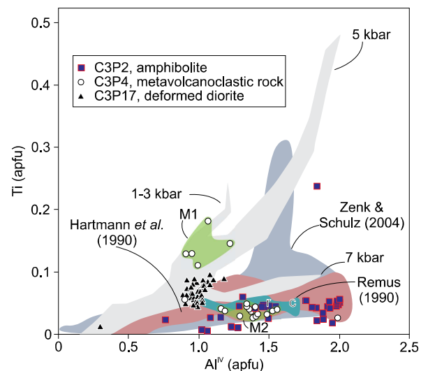
Figure 18. Chemical composition of hornblende ( Al^{IV} ) vs. Ti (apfu) from three studied samples in Zenk and Schulz (2004) diagram, indicating medium pressure metamorphic conditions; M1 in Campestre Formation is suggestive of lower pressure. Published hornblende compositions from São Gabriel terrane also shown. Core (c) and rim (r) of crystals from one amphibolite sample from
