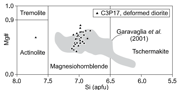
Figure 13. Chemical classification diagram of hornblende from sample C3P17 (deformed diorite) compared with compositions of
