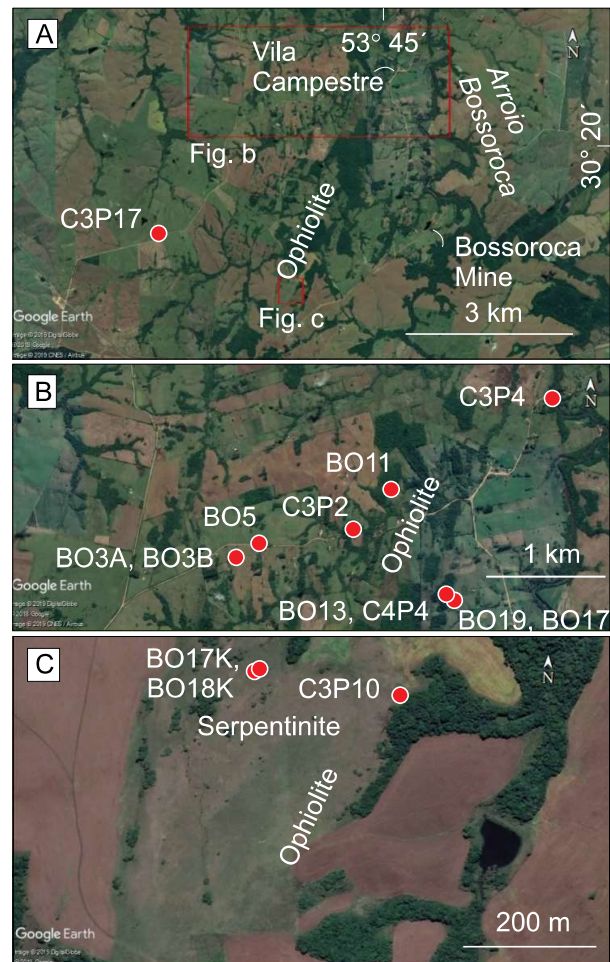
Figure 3. Satellite images of the studied region, northern Bossoroca ophiolite, Campestre transect. Location of studied samples
