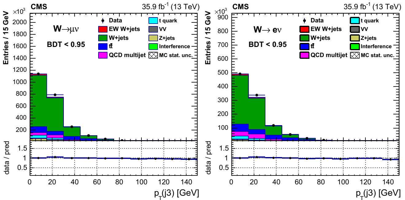
Fig. 23 Leading additional jet p_T ( p_T(j_3) ) for \text{BDT} < 0.95 in the muon (left) and electron (right) channels. In all plots the first bin contains events where no additional jet with p_T > 15 GeV is present
