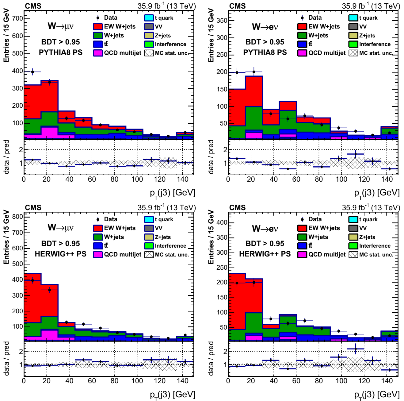
Fig. 15 Leading additional jet p_T ( p_T(j_3) ) for BDT > 0.95 in the muon (left) and electron (right) channels including the signal prediction from MADGRAPH5_aMC@NLO interfaced with PYTHIA parton shower-
