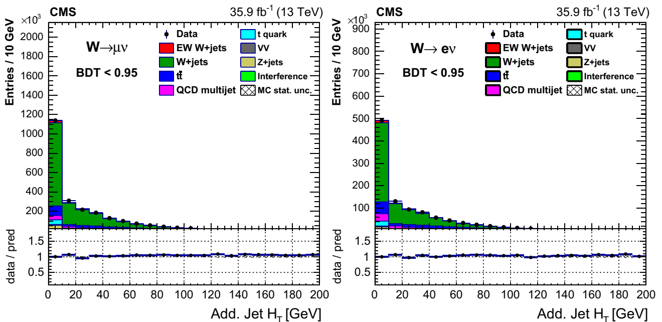
Fig. 24 Total H_T of the additional jets for \text{BDT} < 0.95 in the muon (left) and electron (right) channels. In all plots the first bin contains events where no additional jet with p_T > 15 GeV is present
