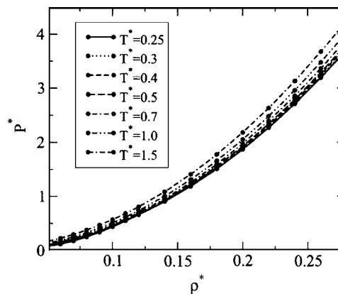
FIG. 3. The reduced pressure as a function of the reduced density. The seven isotherms show that the relation between P^* and \rho^* is monotonic.
