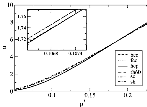
FIG. 2. The dimensionless configurational energy per particle for the several crystal structures considered: face centered cubic (fcc), body centered cubic (bcc), simple cubic (sc), simple hexagonal (sh), hexagonal closest packing (hcp), and rhombohedral-60° (rh60). We see that the hcp has the lower configuration energy per particle for densities \rho^* \leq 0.107 (see inset). Hence, the expected structure for our model at T^* = 0 is the hcp for \rho^* \leq 0.107 . For 0.107 \leq \rho^* \leq 0.187 the bcc phase has the lower configuration energy between those studied (not shown).
