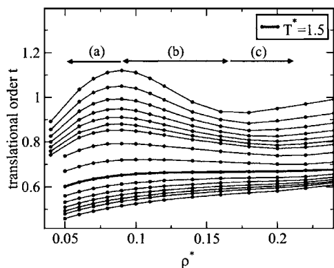
FIG. 4. The translational order parameter t as a function of the density \rho^* . From top to bottom, the 16 isotherms are T^* = 0.25, 0.30, 0.35, 0.40, 0.45, 0.50, 0.55, 0.70, 1.0, 1.5, 2.0, 2.5, 3.0, 3.5, 4.0, and 5.0 . The arrows (a), (b), and (c) correspond to the density range spanned by Figs. 5(a)–5(c), respectively. The bold line indicates the isotherm T^* = 1.5 . For T^* > 1.5 no anomalous behavior is observed for t . The line connecting the points is just a guide for the eyes.
