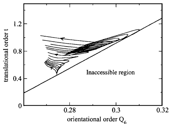
FIG. 8. The t - Q_6 plane or order map. Each line corresponds to an isotherm and the arrows indicate the direction of density growth. From top to bottom, the isotherms showed here are T^* = 0.25, 0.3, 0.35, 0.4, 0.45, 0.5, 0.55, 0.7, 1.0, 1.5, 2.0, 2.5, 3.0, 3.5, 4.0, and 5.0 . Unlike the SPC/E water (Ref. 8), the paths formed by the t and Q_6 parameters developed a two dimensional region in the order map for temperatures and densities inside the structural anomalous region.
