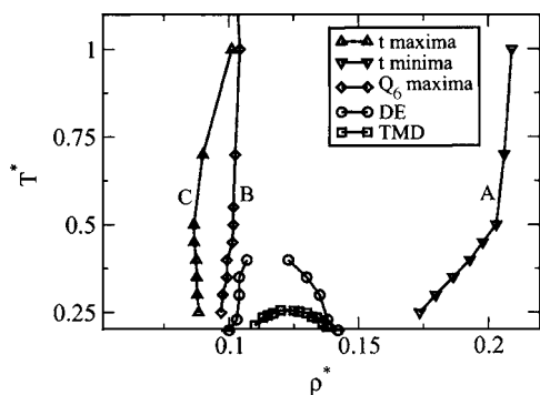
FIG. 7. The relationship between the several anomalies presented for our model. Curve B ends at T^*\approx 5.0 and it is not entirely shown for clarity. See the text for more details. Between the Q_6 maxima line (curve B) and t minima line (curve A) both the translational and orientational order parameters t and Q_6 become anomalous, namely, decrease with density. We call this region the structural anomaly region. The diffusion extrema (DE) lines enclose the region inside which the diffusion decreases with density—the dynamic anomaly region. The temperature of maximum density (TMD) line englobes the region that density anomaly appears. Both the DE and TMD lines were obtained from previous work (Ref. 43). This cascade of anomalies presents the same hierarchy as that observed for the SPC/E water (Refs. 8 and 9).
