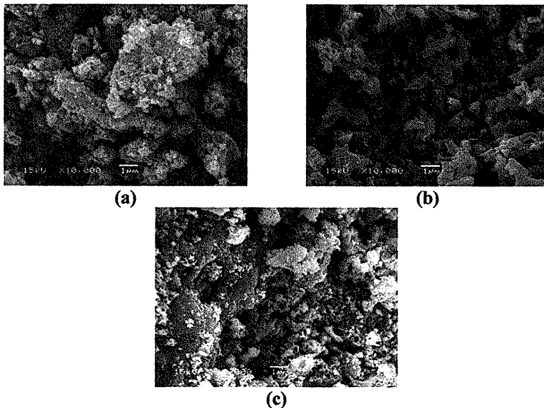
Fig. 6. SEM micrographs of nickel oxide powders prepared by (a) fuel-lean (0.09), (b) stoichiometric (0.37) and (c) fuel-rich (1.11), all at 10,000X magnification.
