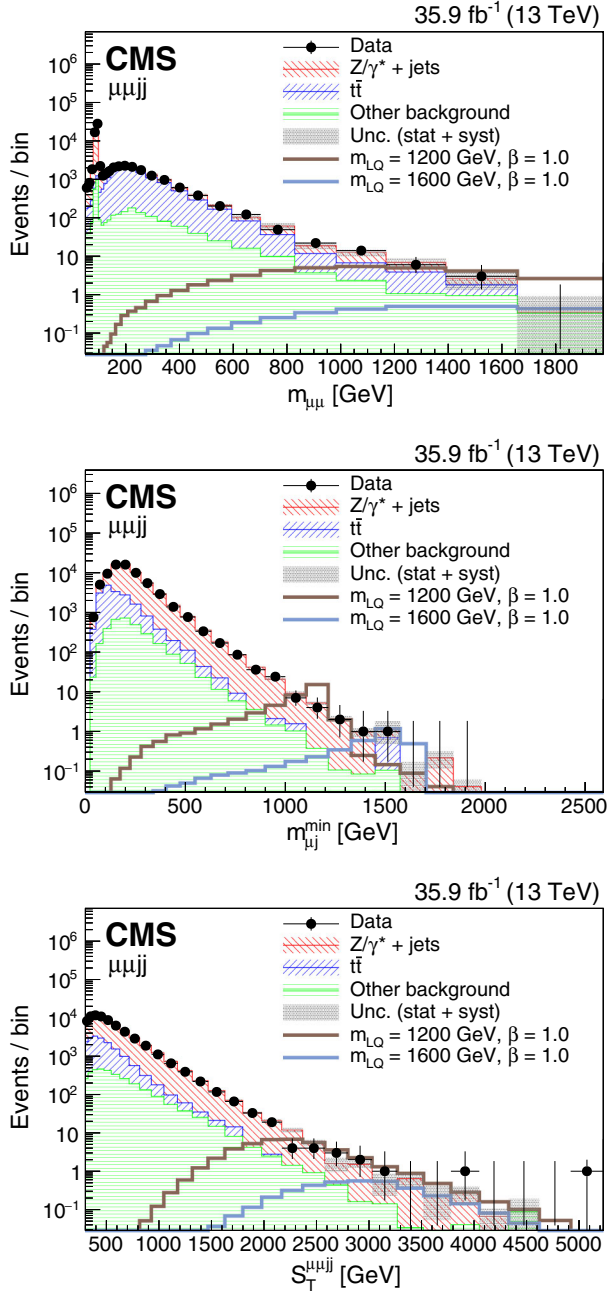
FIG. 2. Comparison of data and background at the preselection level for the \mu\mu jj channel, for the variables used for the final selection optimization: m_{\mu\mu} (upper), m_{\mu j}^{\text{min}} (middle), and S_T^{\mu\mu jj} (lower). “Other background” includes W + \text{jets} , single top quark, and diboson backgrounds. The hashed band represents the combined statistical and systematic uncertainty in the full background estimate.
