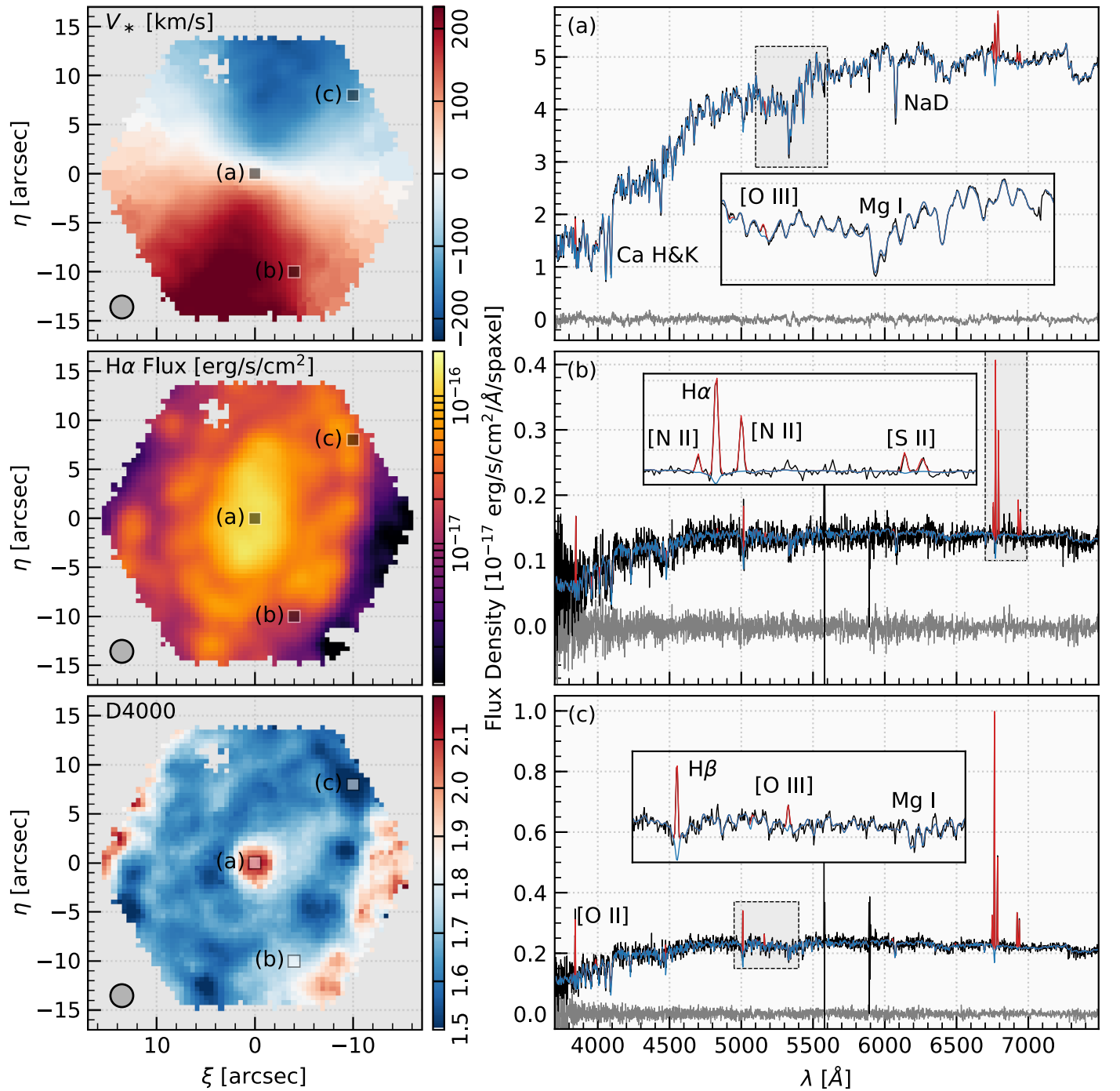
Figure 4. Example data provided by the MaNGA data analysis pipeline (DAP) for MaNGA observation 8138-12704, MaNGA ID 1-339041, following the hybrid-binning approach (DAPTYPE is HYB10-GAU-MILESHC). The left columns shows maps, or images, of some of the DAP-derived quantities, namely, from top to bottom, the stellar velocity field, H \alpha flux, and D4000 spectral index, where the measured value is indicated by the colorbar to the right of each map panel. The effective beam size for the MaNGA observations (FWHM \sim 2''5 ) is shown by the gray circle in the bottom left of each map panel. Three spaxels are highlighted and labeled (a), (b), and (c), according to their spectra plotted in the right column. Each spectrum panel shows the observed MaNGA spectrum (black), stellar-continuum-only model (blue), and best-fitting (stars+emission lines) model (red); the residuals between the data (black) and the model (red) are shown in gray. Note that the red and blue lines are identical except for regions with nebular emission. A few salient emission and absorption features are marked in each panel. Inset panels provide a more detailed view of the quality of the fitted models in the regions highlighted by gray boxes. The spectrum panels only show the spectral regions fit by the DAP, which is limited by the MILES spectral range for DR15.
