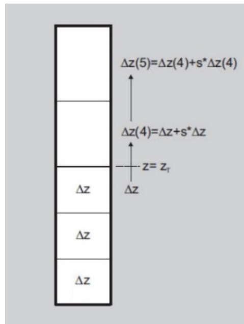
Figure 4.17: The telescoping grid model in ENVI-met 4.0.3, starting after z = z_r 46 (Bruse et al., 2017)
