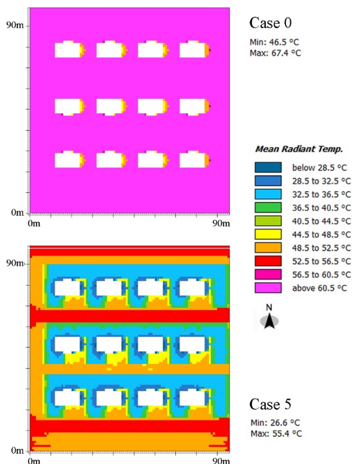
Figure 6.5: T_{mrt} for the Original roofs in the Original site (Case 0) vs. the Green roofs in the Dense green site (Case 5) at 15:00h, at pedestrian level, in the Typical summer day
