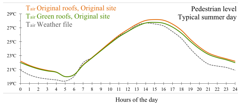
Figure 6.1: T_{air} for Original roofs in the Original site (Case 0) and Green roofs in the Original site (Case 3), at pedestrian level, compared to T_{air} from the weather file, in the Typical summer day
