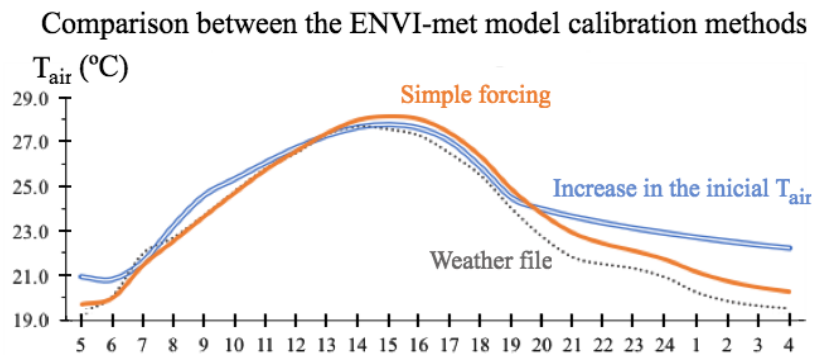
Figure 4.15: Results of T_{\text{air}} with two ways of model calibration, for Case 0: increase in the initial T_{\text{air}} and use of simple forcing, and T_{\text{air}} from the weather file, during a 24-hour period (Typical summer day).
