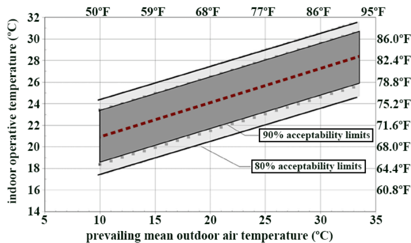
Figure 4.8: Acceptable operative temperature ( T_{op} ) ranges for naturally conditioned spaces (Based on ASHRAE, 2013)
