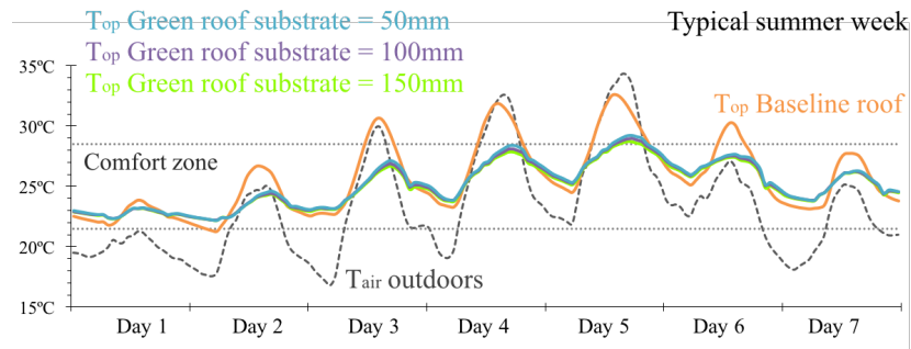
Figure 5.10: Indoor T_{op} for 50mm, 100mm and 150mm of substrate depth and Baseline roof, compared to outdoor T_{air} in the Typical summer week
