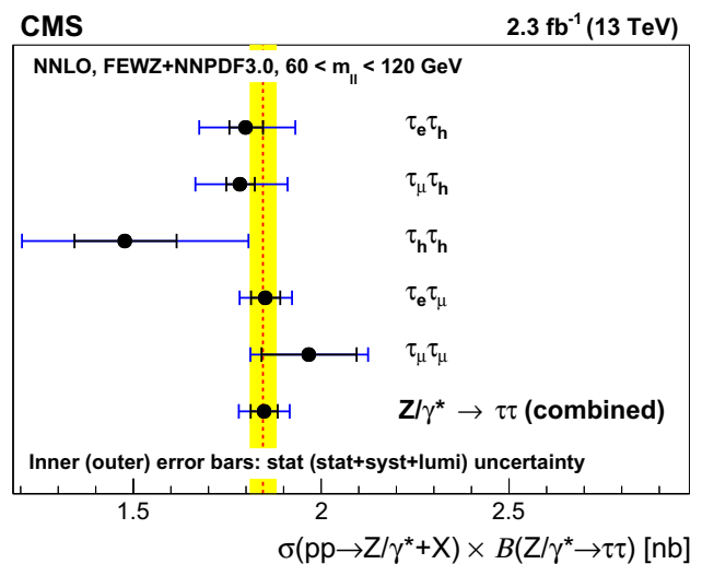
Fig. 12 The inclusive cross section \sigma(pp \rightarrow Z/\gamma^*+X) \mathcal{B}(Z/\gamma^* \rightarrow \tau\tau) measured in individual channels, and in the combination of all final states, compared to the theoretical prediction [60]
