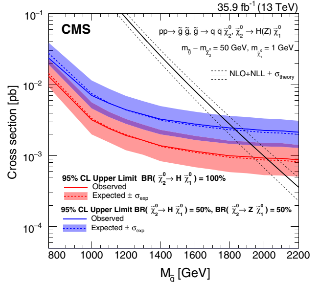
FIG. 3. Observed and expected cross section upper bounds at 95% CL for the T5HH and T5HZ models. The solid and dashed black lines show the SMS gluino-gluino production cross section with its uncertainty. The solid red (blue) line shows the observed limit for the T5HH (T5HZ) model; for each the like-colored dashed line and shaded band show the expected limit and the range associated with the experimental uncertainties.
