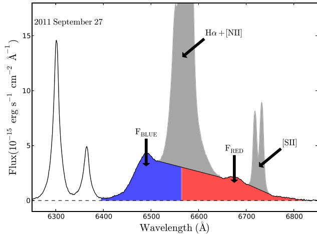
Figure 3. The measured characteristics of the broad double-peaked H\alpha profile F_{\text{Blue}} and F_{\text{Red}} . The grey regions are emission lines that were removed before measuring the flux of the double-peaked profile. The blue region, between 6395 Å and 6563 Å shows the area integrated to obtain the flux of the blue side of the profile, F_{\text{Blue}} . The red region, between 6563 Å and 6820 Å, shows the same for the red side of the profile, F_{\text{Red}} .
