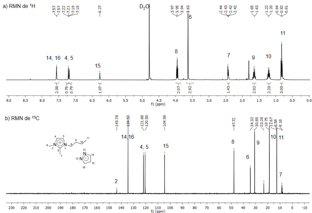
Figura A5. Espectros de RMN do BMMI-Pir em \text{D}_2\text{O} : (a) RMN de ^1\text{H} (400 MHz) e (b) RMN de ^{13}\text{C}\{-^1\text{H}\} (100 MHz).
