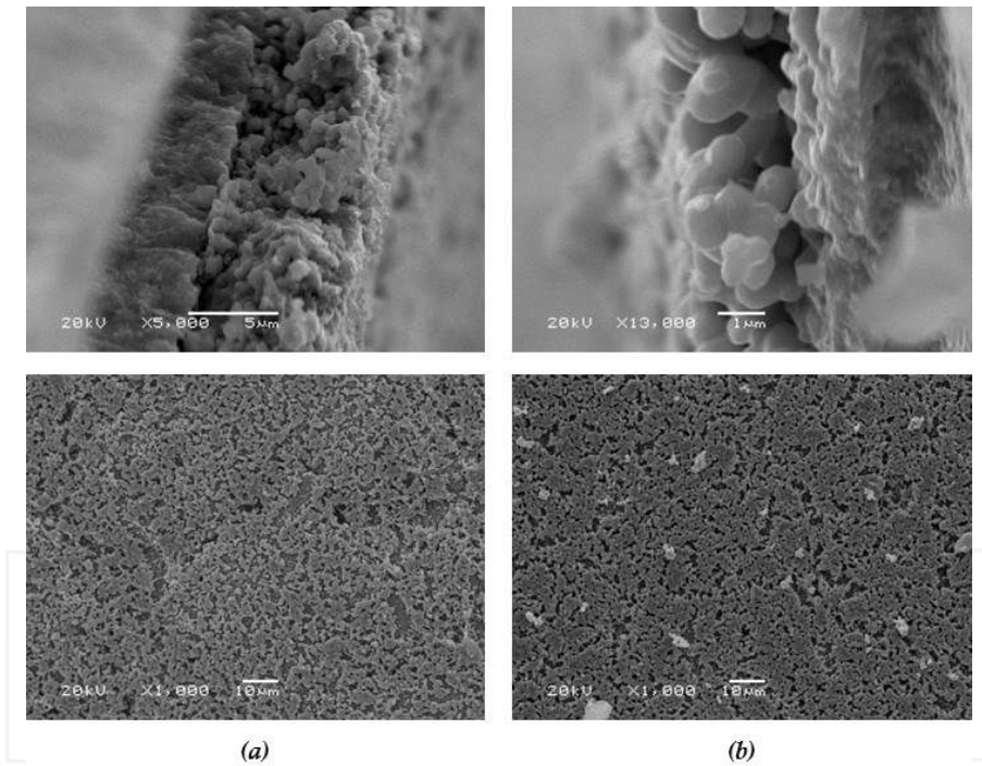
Figure 2. LSM films obtained on YSZ substrates by dip coating with different solutions.
