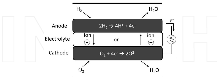
Figure 1. General operation scheme of a fuel cell running with H_2 .
