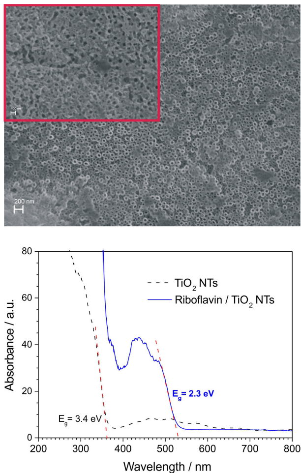
Figure 1. Top view SEM images of a typical TiO 2 nanotube (NT) array grown in an ETG/ammonium fluoride solution (top) and TiO 2 NTs impregnated with RF (inset, error bar: 100 nm). UV-Vis absorption coefficient spectra calculated from diffuse reflectance measurements corresponding to anodic pure TiO 2 NTs and with the impregnation of RF (bottom).
