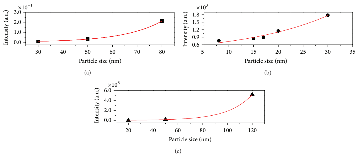
FIGURE 9: Integrated fluorescence intensity, including only the green and red upconverted emission as a function of the nanocrystals average diameter for (a) \text{BaTiO}_3:\text{Er}^{3+} [18], (b) \text{BaYF}_5:\text{Yb}^{3+}/\text{Er}^{3+} [19], and (c) \text{Y}_2\text{O}_3:\text{Er}^{3+} [20].
