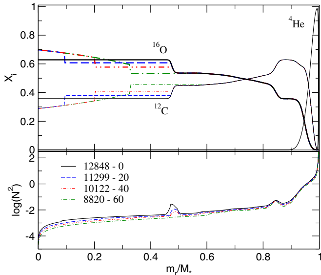
Figure 2. Internal chemical profiles (upper panel) and the logarithm of the square of the Brunt–Väisälä frequency (lower panel), in terms of the mass coordinate, corresponding to a DA white dwarf model with 0.998 M_{\odot} at different stages of the cooling evolution. In this case, we consider the energy release of latent heat and phase separation upon crystallization according to Horowitz et al. (2010). Thick lines depict the oxygen chemical distribution, while thin lines depict the carbon abundance profile. For each model, the effective temperature and percentage of crystallized mass are indicated.
