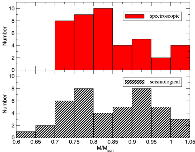
Figure 7. Histograms depicting the mass distribution for the sample of 42 ZZ Ceti massive stars with carbon–oxygen core, studied in this work, according to our spectroscopic (upper panel) and seismological (lower panel) analysis.
