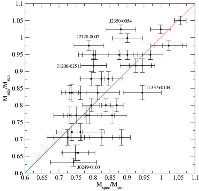
Figure 6. Comparison between the values of the stellar mass according to spectroscopy and asteroseismology. The uncertainties in the asteroseismological mass are the internal uncertainties of the fitting procedure. The red line represents the 1:1 correspondence.
