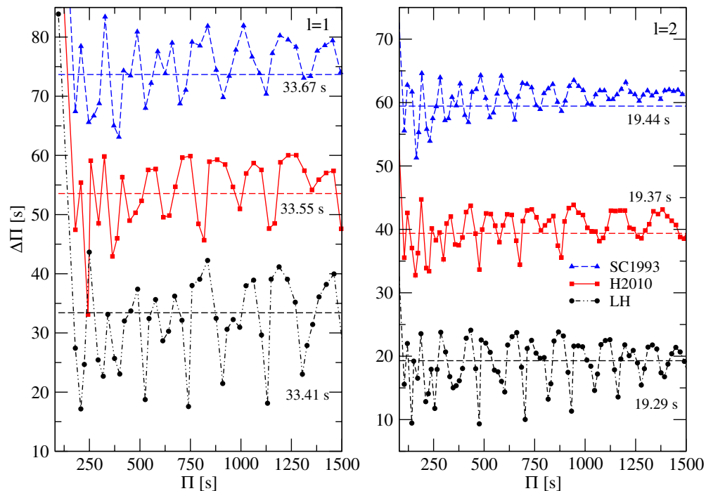
Figure 4. Theoretical period spacing in term of the periods for models with M_* = 0.998 M_\odot and T_{\text{eff}} = 11,600 K for modes with \ell = 1 (left panel) and \ell = 2 (right panel). We show our results obtained by considering only the release of latent heat (black circles) and by using the SC1993 (blue triangles) and H2010 (red squares) phase diagrams. The value of the asymptotic period spacing (horizontal lines) is indicated in each case. The curves are shifted upward in 20 s from the one below, except for the bottom curve.
