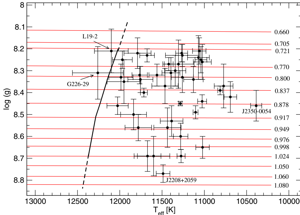
Figure 5. Location of the 42 ZZ Ceti stars analyzed in this paper in the spectroscopic \log g - T_{\text{eff}} plane. The thin red lines correspond to our set of DA white dwarf evolutionary tracks with thick (canonical) H envelope thickness and stellar masses ranging from 0.660 M_{\odot} to 1.080 M_{\odot} . The thick line depicts the theoretical blue edge of the instability strip for massive DA white dwarf stars (see text for details).
