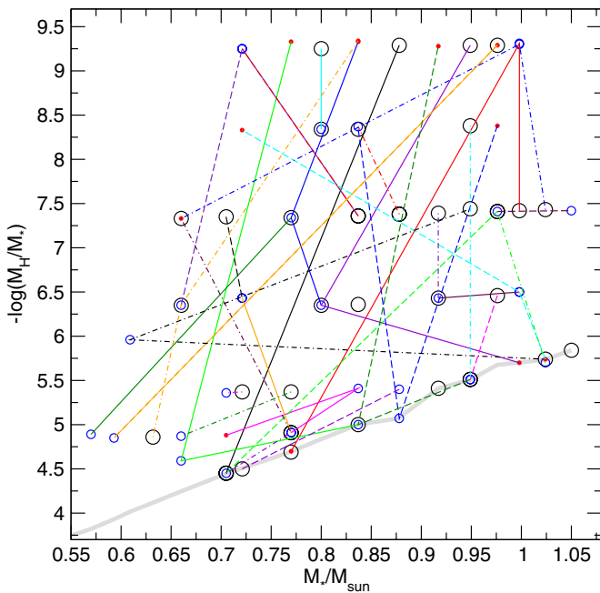
Figure 10. Values of the hydrogen envelope mass in terms of the stellar mass corresponding to all the asteroseismological models of the 42 massive ZZ Ceti stars studied in this work. Large black, medium blue and little full red circles correspond to the first, second, and third asteroseismological solution, respectively, for each star (see Tables 5 and 6). Solutions corresponding to the same object are joined together. The thick, orange line depicts the canonical values of the hydrogen envelope thickness.
