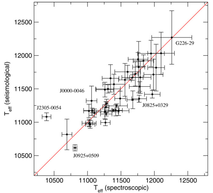
Figure 8. Comparison between the spectroscopic ( x -axis) and seismological ( y -axis) determination of effective temperature for our sample of 42 DAV stars. The red line indicates the 1:1 correspondence.
