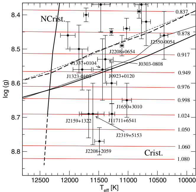
Figure 11. Zoom of Figure 5 on the region where crystallized DA white dwarf should be. The evolutionary tracks used in our study are shown as red lines along with its value of the stellar mass. The thick, full (dashed) lines indicate the limit by crystallization (Crist.) and no-crystallization (NCrist.) for the H2010 (SC1993) phase diagram corresponding to models with canonical H envelopes, and thin lines are for models with the thinner H envelope of each sequence. (A color version of this figure is available in the online journal.)
