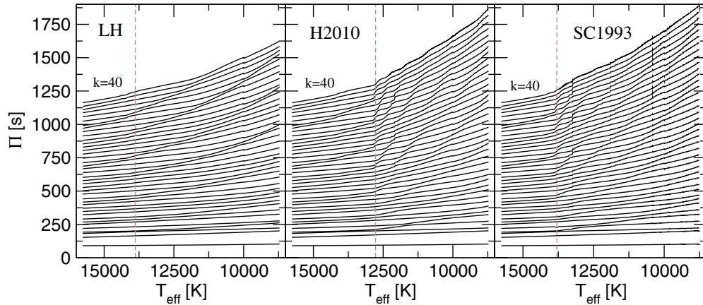
Figure 3. Evolution of the periods for \ell = 1 modes with k = 1-40 as a function of the effective temperature, corresponding to a sequence with M_* = 0.998 M_\odot and canonical H envelope. Left panel: model where phase separation upon crystallization was neglected. Middle panel: result for H2010 phase diagram. Right panel: computation considering SC1993 phase diagram. The vertical line shows the value of T_{\text{eff}} when crystallization sets in.
