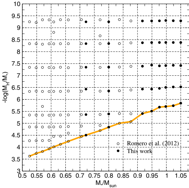
Figure 1. Grid of 163 DA white dwarf evolutionary sequences considered in this work in the M_* – \log(M_H/M_*) plane. Each circle corresponds to a sequence of models representative of white dwarf stars characterized by a given stellar mass and hydrogen envelope mass. Open circles correspond to the evolutionary sequences computed in Romero et al. (2012), while filled circles correspond to sequences computed in this work. The orange thick line connects the sequences with the maximum values for the thickness of the hydrogen envelope, predicted by our evolutionary computations.
