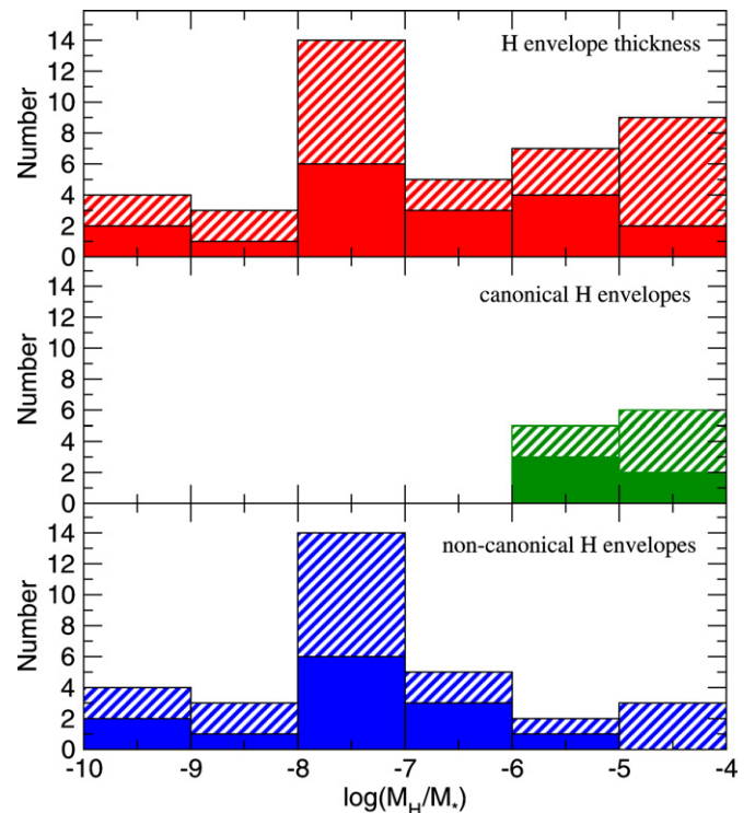
Figure 9. Upper panel: histogram showing the hydrogen envelope thickness distribution for our complete sample of 42 massive DAV stars (dashed). Middle panel: histogram for models with canonical values of the hydrogen envelope thickness, as predicted by stellar evolution theory for each mass. Lower panel: histogram for models with non-canonical values of the hydrogen envelope thickness, as obtained by means of our artificial procedure described in Section 2.2. We consider only the best-fit model solutions for each star. In addition, with fill bars, we show the results corresponding to a sample composed only with stars having three or more modes in their spectrum (see Table 5).
