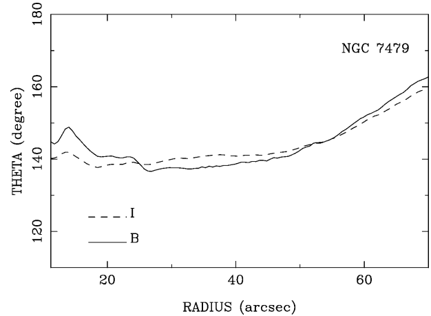
FIG. 3.—Relative behavior of the two-armed phase \Theta_B(r) and \Theta_I(r) for NGC 7479. The diagram indicates the presence of two CRs at r \approx 23'' and r \approx 55'' . The SDW is trailing around the inner CR and leading around the outer one.
