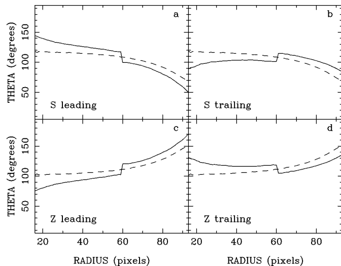
FIG. 2.—Relative behavior of the phase \Theta(r) of the SDW ( dashed line ) and the shock front ( solid line ) for the four cases shown in Fig. 1.
