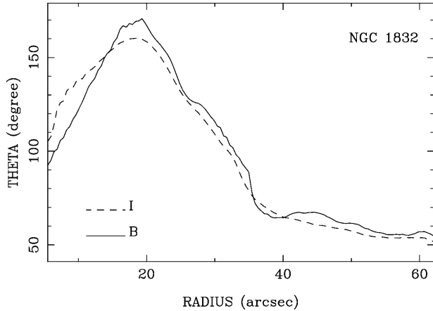
FIG. 5.—Relative behavior of the phases \Theta_B(r) and \Theta_I(r) for NGC 1832. The diagram indicates the presence of three CRs at r \approx 15'' , r \approx 34'' , and r \approx 40'' . The SDW is leading around the inner and the outer CRs, and it is trailing around the intermediate one.
