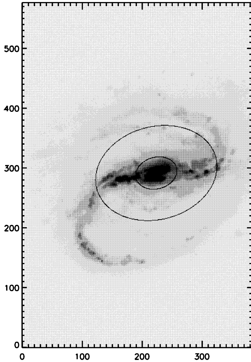
FIG. 4.—CR circles on a NGC 7479B image. North is at the top, and east is to the left. Scales are in pixels, 1 pixel = 0''.560 ; V_R = 2378 \text{ km s}^{-1} .
