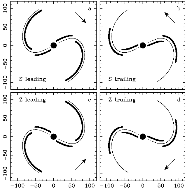
FIG. 1.—The position of the shock front ( heavy line ) with respect to the SDW ( light line ) for (a) leading, S-type wave; (b) trailing, S-type wave; (c) leading, Z-type wave; (d) trailing, Z-type wave. The arrow in each panel indicates the sense of the disk rotation. Note: An S-type object would be seen as a Z-type if viewed from the opposite pole of its axis of rotation. The distinction is observational rather than physical.
