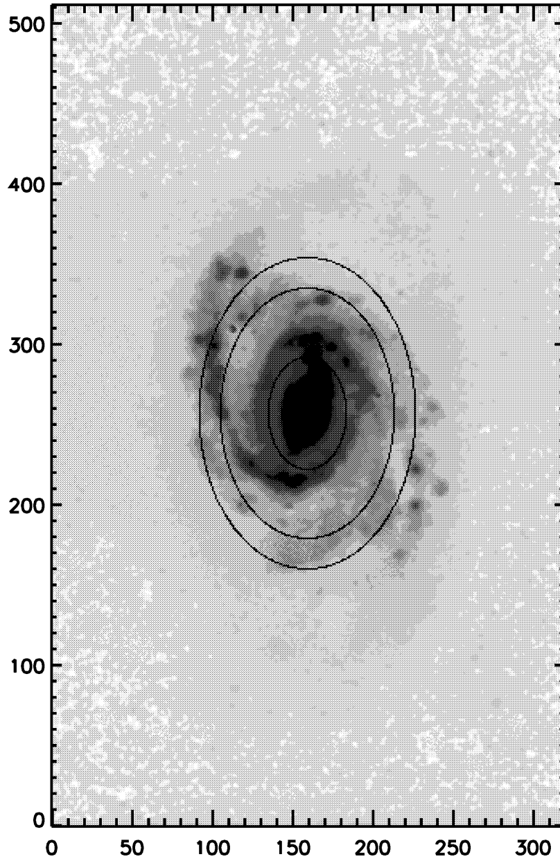
FIG. 6.— B image of NGC 1832 showing the position of the three CRs. North is at the top, and east is to the left. Scales are in pixels, 1 pixel = 0''.414 ; V_R = 1937 km ^{-1} .
