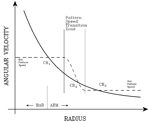
FIG. 7.—Schematic diagram for NGC 1832 showing the possible relative behavior of the disk (solid line) and the perturbing pattern (dashed line) angular velocities.
