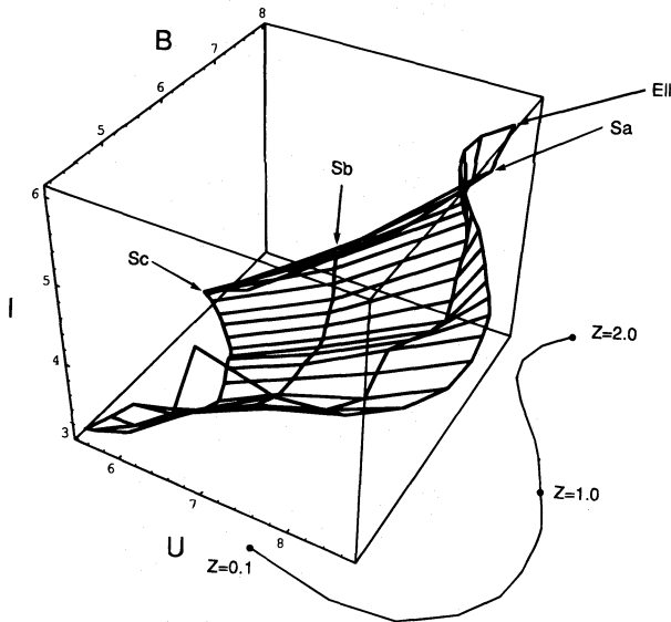
FIG. 4.— U , B , and I magnitudes are shown for the normal galaxy templates as a function of redshift, from z = 0 to z = 2 . The grid shows the magnitudes for the elliptical, Sa, Sb, and Sc templates as four lines defining a curved surface. Lines of equal redshift, in increments of 0.1, are drawn perpendicular to the four lines. The galaxies have been normalized in the red. The curved line to the right of the cube shows the path of the elliptical galaxy template with redshift z = 0.1 , z = 1.0 , and z = 2.0 marked.
