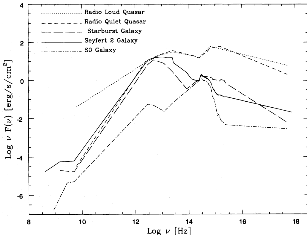
FIG. 5.—SED for the S0 galaxy NGC 1553, for the starburst galaxy NGC 7714, and for the Seyfert 2 galaxy NGC 1068 normalized at 1.2 \mu\text{m} , overlaid with a template radio-loud quasar and radio-quiet quasar from Sanders et al. (1989). The quasars are normalized to the Seyfert 2 galaxy by the flux in the IRAS band at 60 \mu\text{m} , a flux that is thought to be isotropic and therefore not dependent on the orientation angle of the active nucleus.
