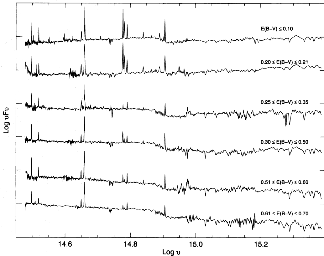
FIG. 13.—Templates of starburst galaxies plotted in the same units as Figs. 10 and 11
