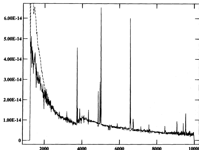
FIG. 9.—The template for the starburst galaxy ( solid line ) with E(B-V) = 0.0 is plotted with a synthetic spectrum overlaid ( dashed line ). The spectra are normalized at 4000 \text{ \AA} . The synthetic spectrum is based on a continuous star formation model of age 7.2 \times 10^8 yr.
