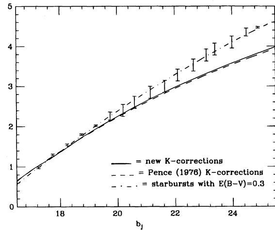
FIG. 7.—Prediction for number counts for the no-evolution galaxy model compared with the data of Broadhurst et al. (1988) as a function of the blue magnitude B_j . Data are given with 1 \sigma error bars. Prediction based on our K -corrections are given by the solid line. Predictions based on Pence (1976) K -corrections are given by the dashed line. For comparison, a prediction based on a highly unphysical universe made up completely of starbursts with low dust content is given by the dot-dashed line.
