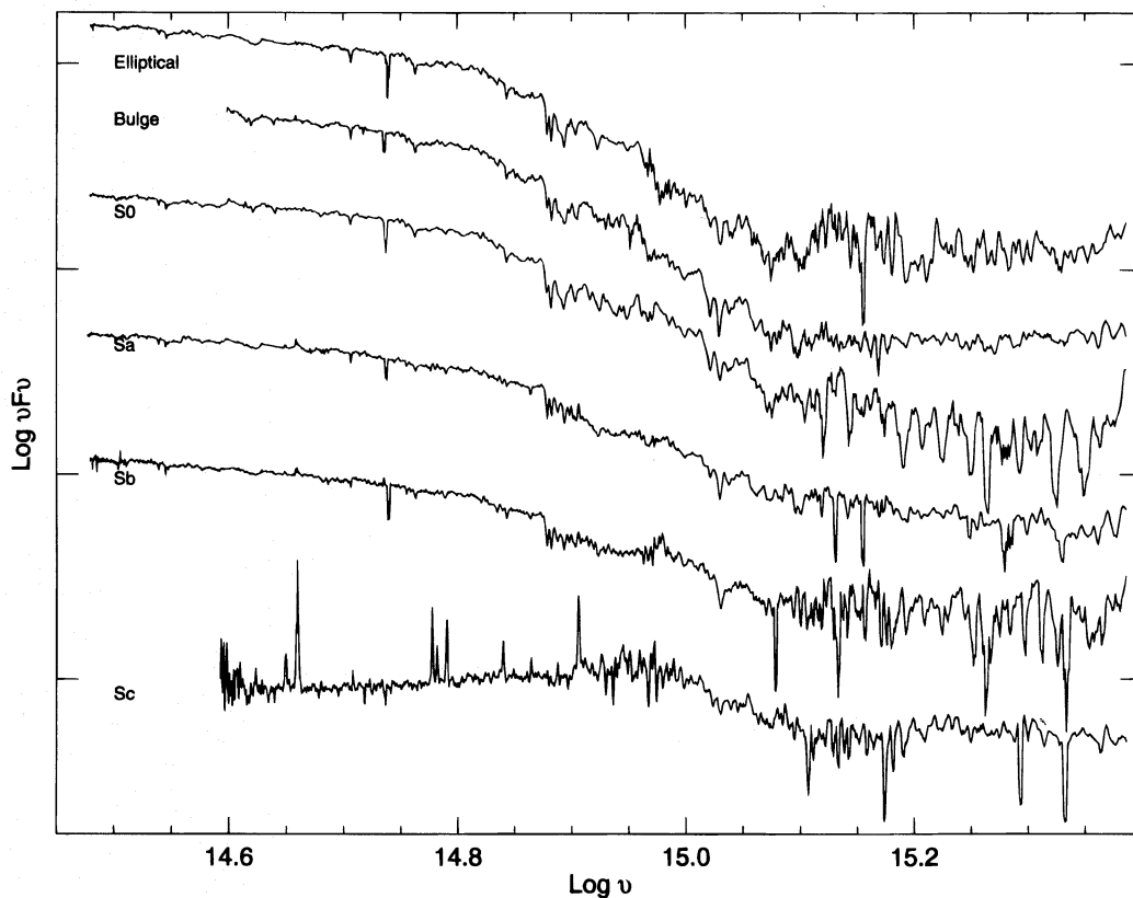
FIG. 12.—Templates of normal galaxies plotted in the same units as Figs. 10 and 11
