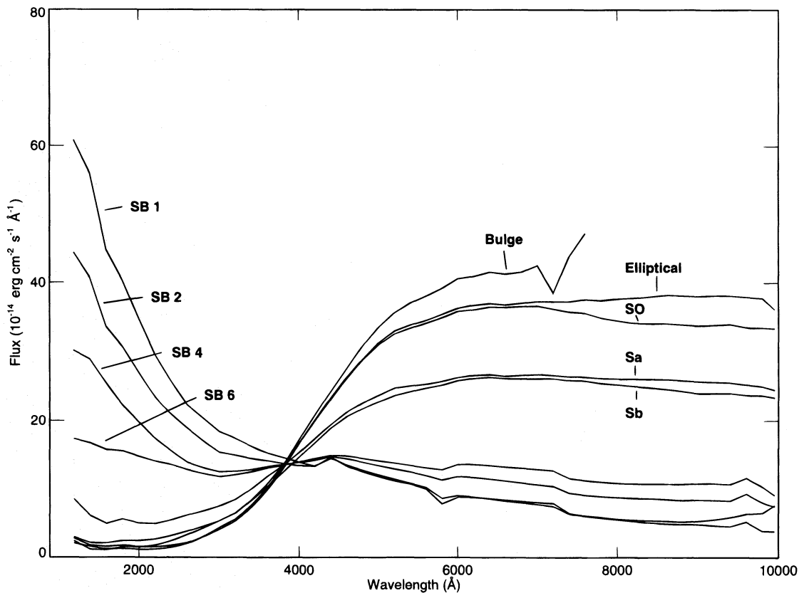
FIG. 1.—The spectra binned in 200 Å bins are shown between 1200 and 10,000 Å, normalized at 4000 Å for the bulge, elliptical, S0, Sa, Sb, and starburst galaxies with varying dust content. The starburst galaxy templates are grouped according to the mean color excess value E(B-V) and are labeled as SB1 for E(B-V) < 0.10 ; SB2 for 0.11 \leq E(B-V) \leq 0.21 ; SB4 for 0.39 \leq E(B-V) \leq 0.50 ; and SB6 for 0.61 \leq E(B-V) \leq 0.70 .
