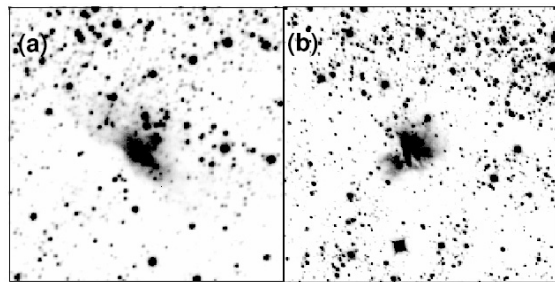
Fig. 3. K_s SOFI large field extractions: a) 2' \times 2' of Object 26 and b) 2' \times 2' of Object 56. North is up and west to the right.
