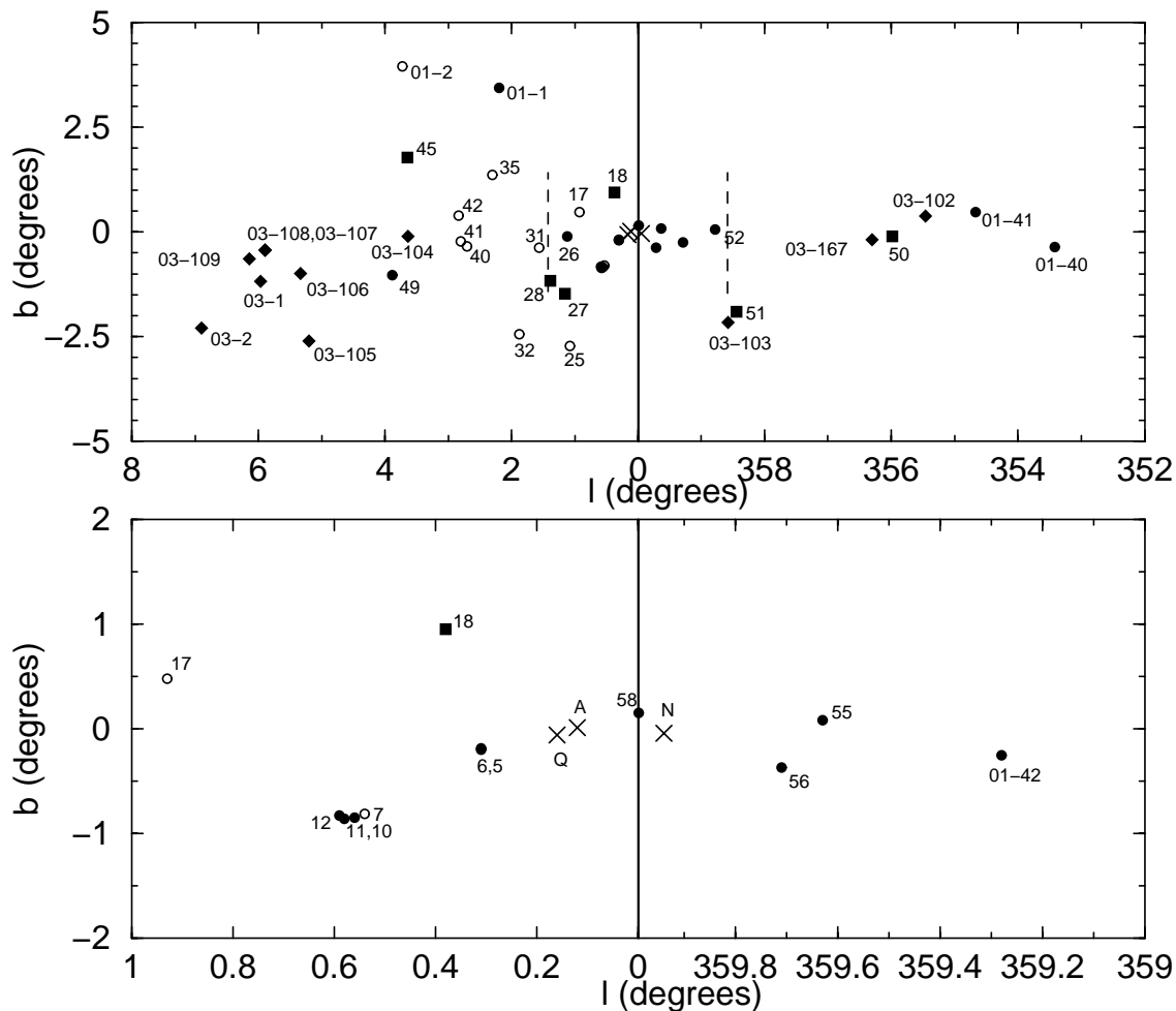
Fig. 5. Upper panel: updated angular distribution of star clusters and candidates in the inner 7'' (1 kpc at the Galactic Center distance). Lower panel: blowup to show in detail the central region within 1'' . Objects from Dutra & Bica (2001) are labeled as 01- and from Bica et al. (2003) as 03-, the other objects are from Dutra & Bica (2000). Crosses are the Arches, Quintuplet and Nuclear Young Cluster. Filled circles are objects from the present study which are confirmed as clusters or candidates. Open circles are dissolving cluster candidates. Filled squares are objects from Dutra & Bica (2000) not included in the present work. Filled diamonds are objects from Bica et al. (2003).
