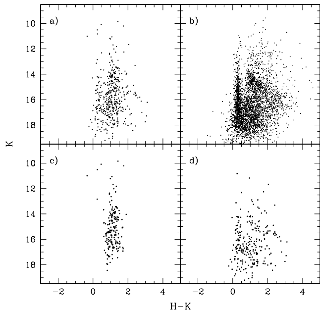
Fig. 9. K, H - K diagrams: a) Object 11 area, extraction of stars with distance r < 43.5'' ; b) bulge field, extraction of stars outside where field stars r > 58'' ; c) clean cluster CMD; and d) stars subtracted from the Object 11 area CMD in order to obtain the decontaminated CMD.
