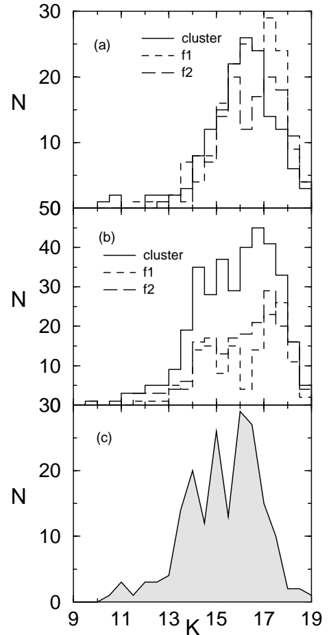
Fig. 8. Upper panel: K histogram for stars in the range 0.0 < H - K < 0.5 . Middle panel: K histogram for stars in the range 0.75 < H - K < 1.5 . Continuous line corresponds to object while dashed and long dashed lines to the fields. Lower panel: K cluster luminosity function derived from average field subtraction for 0.75 < H - K < 1.5 .
