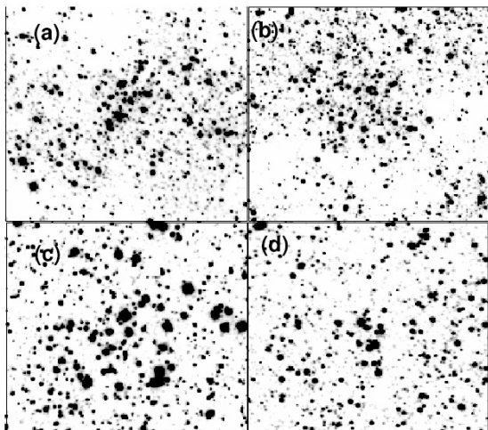
Fig. 4. K_s SOFI large field extractions: a) 2' \times 2' of Object 58, b) 3' \times 3' of Object 01-42, c) 3' \times 3' of Object 01-01, and d) 2' \times 2' of Object 1. North is up and west to the right.
