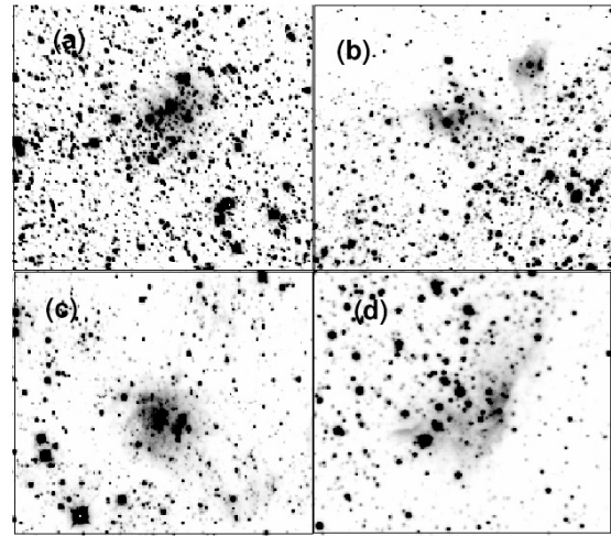
Fig. 2. K_s SOFI large field extractions: a) 2' \times 2' of Object 52, b) 2' \times 2' of Object 6 (centre) and Object 5 (right), c) 2' \times 2' of Object 10, and d) 2' \times 2' of Object 01-41. North is up and west to the right.
