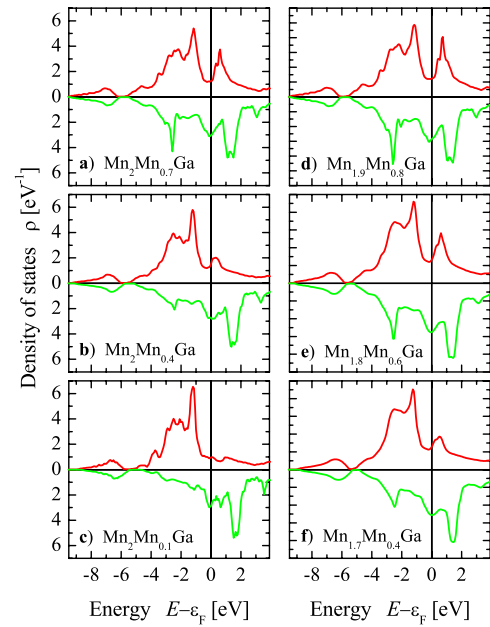
FIG. 4. (Color online) Density of states for Mn_{3-x}Ga . (a)–(c) show the DOS for model I: Mn_2(Mn_{1-x}\square_x)Ga . (d)–(f) show the DOS for model III: (Mn_{2-x/3}\square_{x/3})(Mn_{1-2x/3}\square_{2x/3})Ga . Shown are the selected compositions with x=0.3 [(a) and (d)], 0.6 [(b) and (e)], and 0.9 [(c) and (f)]. Majority densities are shown in the upper parts, and minority states in the lower parts of each of the plots.
