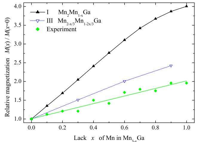
FIG. 11. (Color online) Comparison of magnetization data for \text{Mn}_{3-x}\text{Ga} . The values are normalized to x=0 for better comparison. Experimental values are for an induction field of 5 T. Calculated values for models I and III are seen in Sec. IV A 2.
