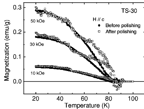
FIG. 6. FCC magnetization for the TS-30 sample measured in the indicated fields as a function of the temperature, before and after polishing its surfaces. Note that the magnetizations are quoted in emu/g to facilitate their quantitative comparison. The magnetic contribution of the Y211 particles is removed.
