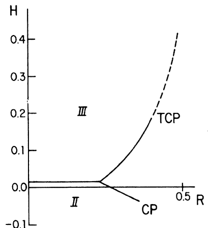
FIG. 1. Typical phase diagram for the three-state Potts model with symmetry-breaking perturbations taken from Ref. 19 and similar to one in BA-I. Dimensionless temperature and field variables, R = (4u_1/9w^2)r and H = (16u_1^2/27w^3)h_1 are used. The solid lines represent first-order transitions ending at a critical point (CP) or a tricritical point (TCP) and the broken line indicates a second-order transition.
