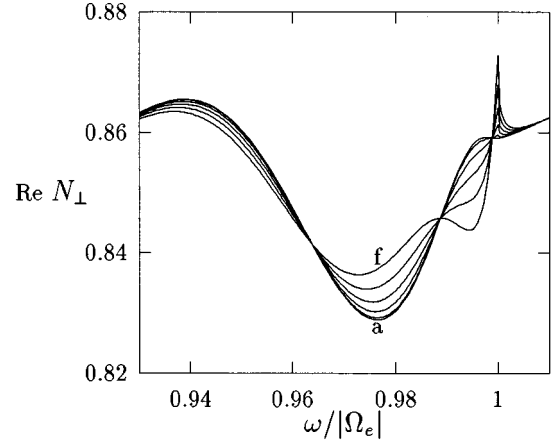
FIG. 1. Real part of the refraction index for ordinary mode waves vs normalized frequency, for several values of the inhomogeneity parameter \tilde{N}_B ( \tilde{N}_B = 0, 2 \times 10^{-3}, 4 \times 10^{-3}, 6 \times 10^{-3}, 8 \times 10^{-3}, and 1 \times 10^{-2} ). Curve a , \tilde{N}_B = 0 ; curve f , \tilde{N}_B = 1 \times 10^{-2} ; the curves corresponding to the other values of \tilde{N}_B appear between the curves indicated by a and f , for increasing \tilde{N}_B . The parameters considered are l_e = 1, T_{\perp} = T_{\parallel} = T_e = 5 keV, X_e/Y_e^2 = 0.5, N_{\parallel} = 0, and \psi = 0 .
