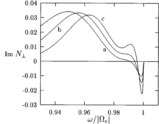
FIG. 4. Imaginary part of the refractive index for ordinary mode waves vs normalized frequency, for curve a , T_e=4 keV; curve b , T_e=5 keV; and curve c , T_e=6 keV. The parameters considered are l_e=1 , X_e/Y_e^2=0.5 , N_{\parallel}=0 , \psi=0 , and \tilde{N}_B=1\times 10^{-2} , for T_{\perp}=T_{\parallel}=T_e .
