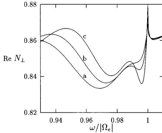
FIG. 3. Real part of the refractive index for ordinary mode waves vs normalized frequency, for curve a , T_e=4 keV; curve b , T_e=5 keV; and curve c , T_e=6 keV. The parameters considered are l_e=1 , X_e/Y_e^2=0.5 , N_{\parallel}=0 , \psi=0 , and \tilde{N}_B=1\times 10^{-2} , for T_{\perp}=T_{\parallel}=T_e .
