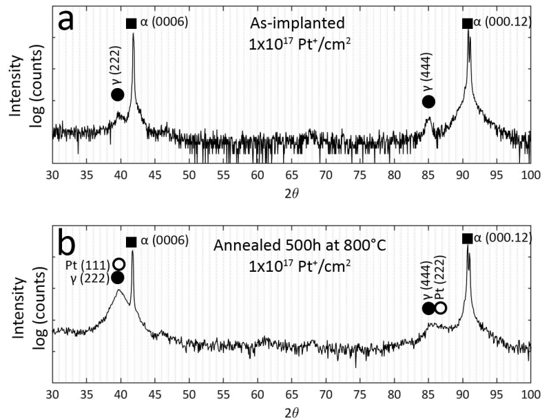
Fig. 2. XRD of sapphire wafers after implantation but before annealing (a) showing intense \alpha - \text{Al}_2\text{O}_3 peaks and broad, weak peaks likely due to a transition alumina formed by implantation damage to the matrix. After 500 h at 800 °C (b), peaks consistent with Pt and a transition alumina are visible. The lack of other peaks is evidence of highly oriented growth of transition alumina and the consistent orientation of the Pt nanoparticles within the alumina. Identification of Pt and \gamma -alumina peaks is based on additional information from TEM imaging and diffraction.
