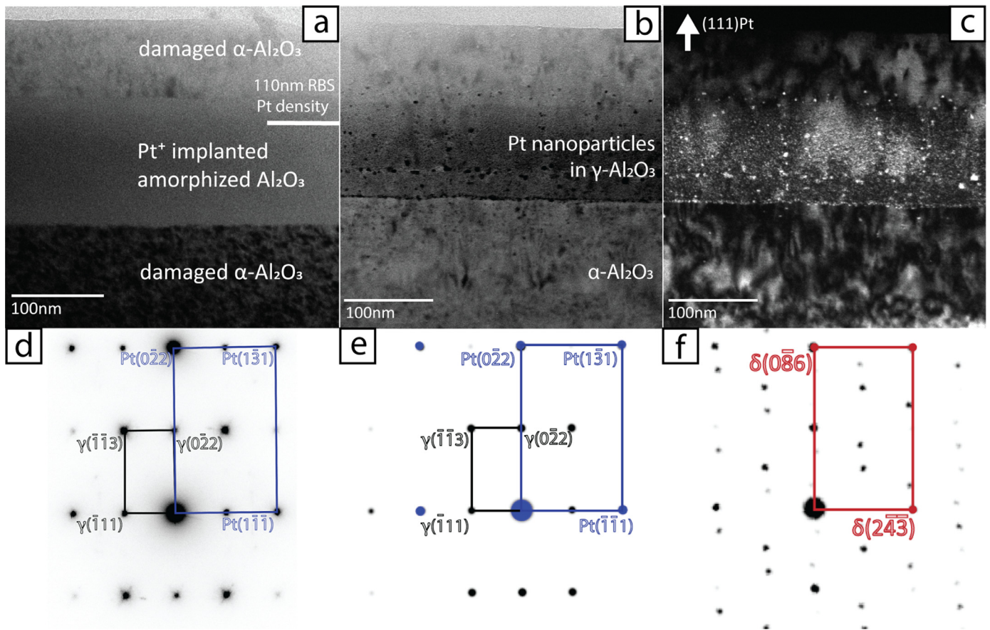
Fig. 3. BF TEM images of a cross section of (a) the as-implanted 5 \times 10^{16} Pt/cm 2 wafer and (b) after 500 h at 800 °C. The sapphire is amorphized where the peak density of implanted Pt occurs. After 500 h at 800 °C (b), the amorphous alumina has recrystallized as \gamma -alumina and the \alpha -alumina has grown into the region that had been amorphized. Most of the precipitates are near the peak of the implanted Pt density, but they also decorate the \gamma/\alpha -alumina boundary. (c) DF image of the region in (b) taken in a two-beam condition from (111)_{Pt} and (222)_{\gamma} ; the smallest objective aperture could not exclude the (0006)_{\alpha} diffracted beam. The DF image highlights the high degree of alignment of the Pt within the \gamma -alumina and of \gamma -alumina with the \alpha phase. Experimental SAED pattern (d) of the implanted region after annealing at 800 °C for 500 h; the adjacent sapphire was excluded with the selected area aperture. The intensities were inverted for clarity. Simulated SAED patterns of (e) Pt and \gamma -alumina along the [211]_{\gamma} zone axes, using the Zhou and Snyder model [12] and (f) of \delta -alumina using a structure reported by Kovarik et al. [17] along the [35.9.12]_{\delta} zone axis where (243)_{\delta} is equivalent to (\bar{1}11)_{\gamma} (parallel to close-packed planes of the oxygen sub-lattice) and (043)_{\delta} is to (022)_{\gamma} .
