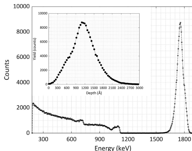
Fig. 1. RBS spectrum used to determine the depth and Pt fluence in the sapphire wafer with a target fluence of 1 \times 10^{17} \text{Pt}/\text{cm}^2 before thermal treatment. The peak concentration of Pt occurred at a depth of 110 nm and fluence was found to vary over the wafer, ranging between 0.8 and 2 \times 10^{17} \text{Pt}^+/\text{cm}^2 .
