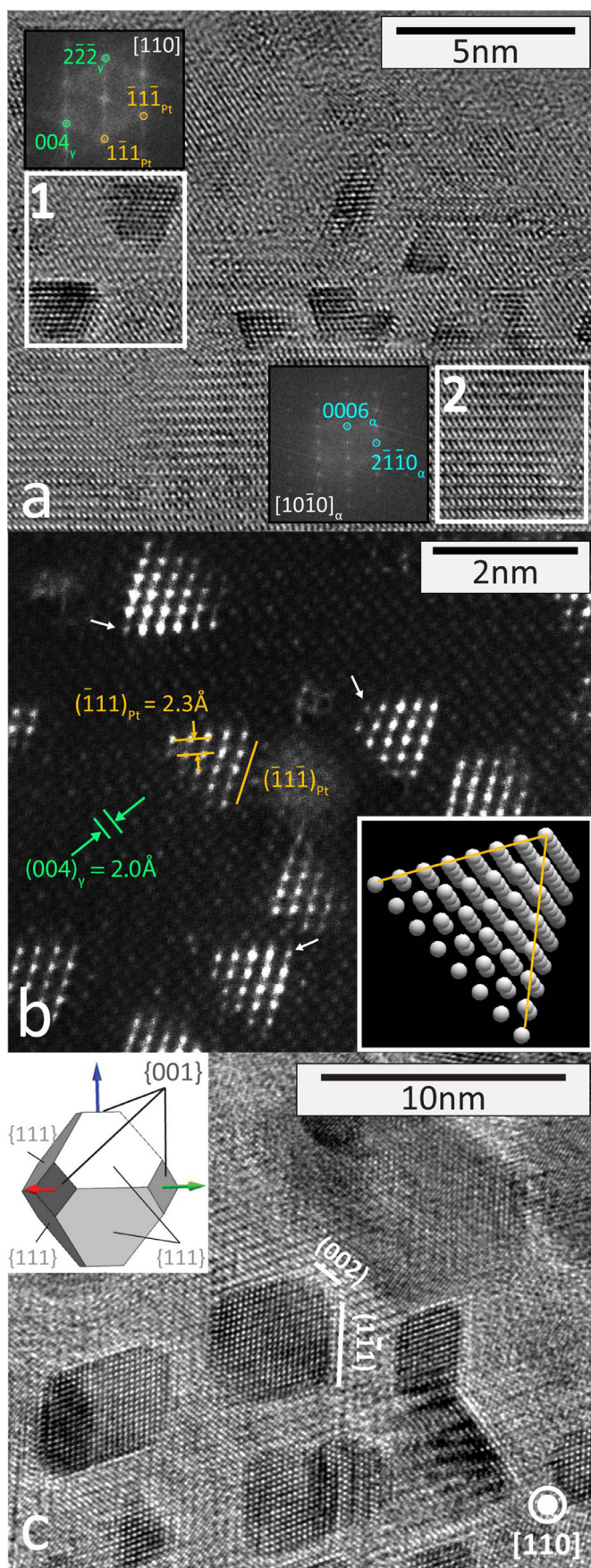
Fig. 4. Aberration-corrected phase-contrast HRTEM (a,c) and probe-corrected HAADF STEM (b) micrographs of the 1 \times 10^{17} Pt/cm 2 implanted wafer after 800 °C at 500 h. The FFT of region 1 in (a) is consistent with the cube-
