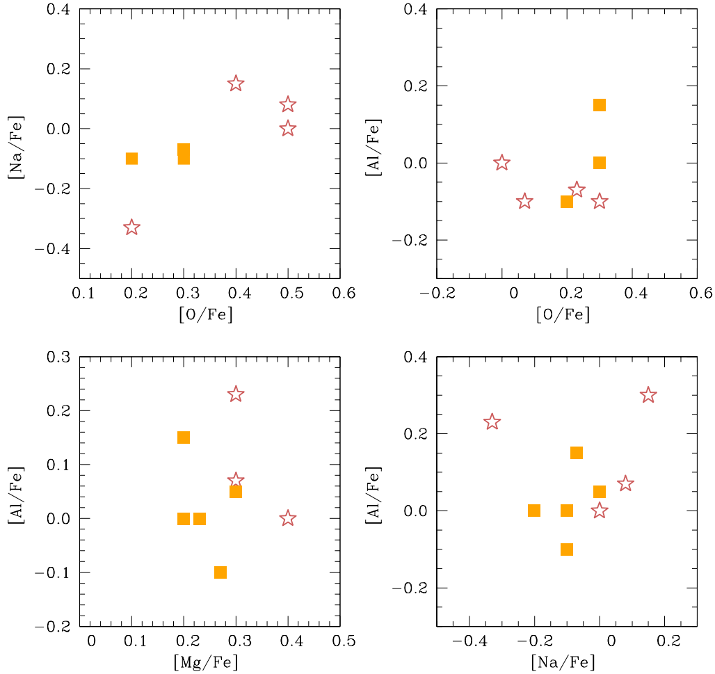
Fig. 9. [Na/Fe] vs. [O/Fe], [Al/Fe] vs. [O/Fe], [Al/Fe] vs. [Mg/Fe], and [Al/Fe] vs. [Na/Fe] for the sample stars: indian red open stars, and Barbuy et al. (2007): orange filled squares.
