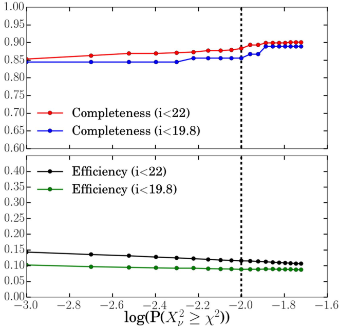
Figure 10. Completeness and efficiency of variability selection P(X_v^2 \geq \chi^2) > 0.01 for the P15-S1S2 Quasar Catalog, where P(X_v^2 \geq \chi^2) is the probability of rejecting the null hypothesis that sources are nonvariable. The dotted line at \log(P(X_v^2 \geq \chi^2)) = -2.00 corresponds to rejecting the null hypothesis at 99% confidence.
