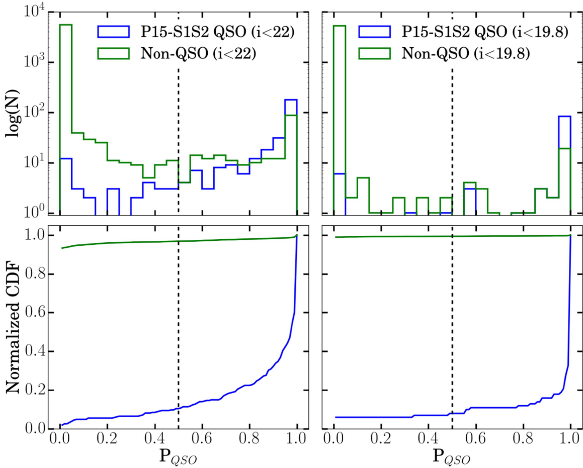
Figure 8. Top panel: distribution of \chi^2_{\text{QSO}} quasar probabilities for the P15-S1S2 quasars and point-source non-quasars with WISE photometry at the faint and bright magnitude limits. The dotted line denotes the probability cut at P_{\text{QSO}} = 0.5 . Bottom panel: the cumulative distribution of the same quasars and non-quasars in P_{\text{QSO}} . The majority (>90%) of the non-quasars have P_{\text{QSO}} < 0.5 while quasars mostly have P_{\text{QSO}} > 0.5 .
