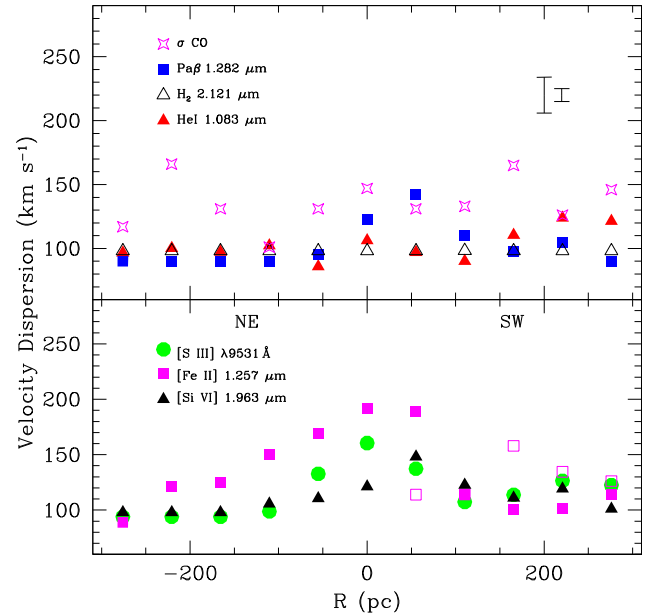
Figure 11. Velocity dispersion derived for the different emission lines observed as well as for the stellar CO band heads. The instrumental velocity resolution is 90 \text{ km s}^{-1} , meaning that H 2 is not resolved spectroscopically in any apertures. The bars at the top right of the plot indicate the maximum and average errors ( 1\sigma ) derived from the measurements. For [Fe II] (bottom panel), filled squares are for the blue component of the line while open squares are for the red component. At 110 pc SW, both components have the same width.
