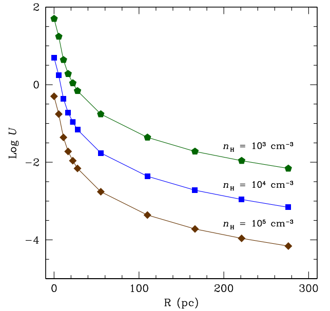
Figure 13. Variation of the log of the ionization parameter, \log U , with the distance from the centre of the AGN for clouds of density n_H = 10^3 , 10^4 and 10^5 cm ^{-3} . The symbols are the same employed in Fig. 12.
