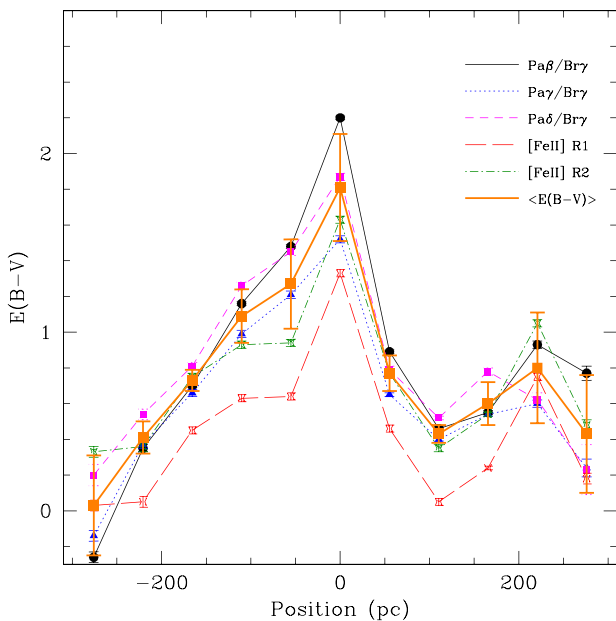
Figure 7. Values of E(B - V) derived from different H II line flux ratios as well as from the [Fe II] 1.257 \mu\text{m} /1.644 \mu\text{m} flux ratio using an intrinsic value of 1.25 (R1, long-dashed line) and 1.36 (R2, dash-dotted line) for the nuclear and off-nuclear apertures of NGC 4388. The thick solid line is the average extinction along the spatial direction. See the text for further details.
