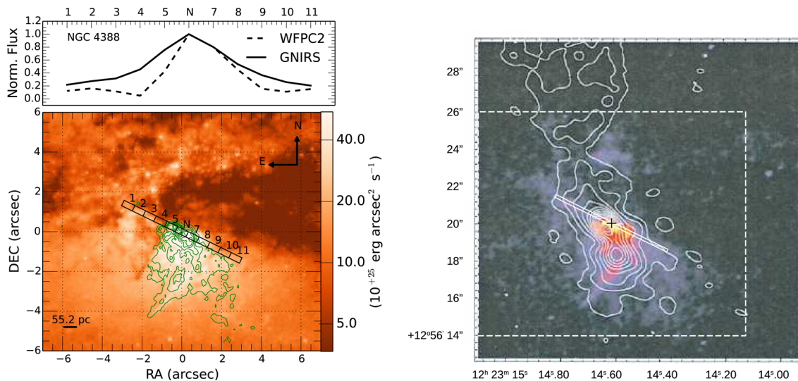
Figure 1. Left: continuum WFPC2/ HST in the F606W filter overlaid on [O III] \lambda 5007 contours (described in Falcke et al. 1998). The GNIRS slit is positioned at an angle of PA=64^\circ and illustrates approximately the region covered by the NIR spectra. ‘N’ marks the position of the nuclear aperture while the numbers 1 to 5 and 7 to 11 denote the off-nuclear extractions. The two curves on top show the light profile along the spatial direction of the slit for the GNIRS spectrum (black solid line) and in the [O III] image at the same PA as the slit (dashed line). North is up and east is to the left. The spatial scale is indicated by the bar at the bottom-left corner and represents the size of the aperture window used in extracting the spectra. Right: H\alpha image from WFPC2/ HST overlaid on radio contours as originally published by Falcke et al. (1998). The thick white box represents the GNIRS slit while the dashed square marks approximately the field covered by the image to the left. The black cross is the position of the optical nucleus.
