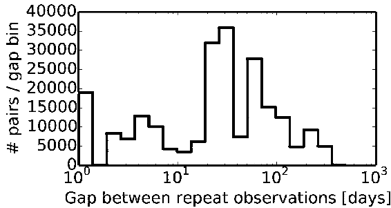
Figure 5. Distribution of time between visits for APOGEE stars, useful for determining the sensitivity to radial velocity variations due to binarity. This quantity is the absolute value of the time difference for all unique pairs of visits for each star. The most prominent peaks are at 1 and 2 months.
