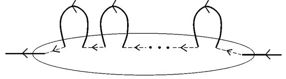
FIG. 2. Generic diagram of G_{ii\sigma} for the FK model in d=\infty .
