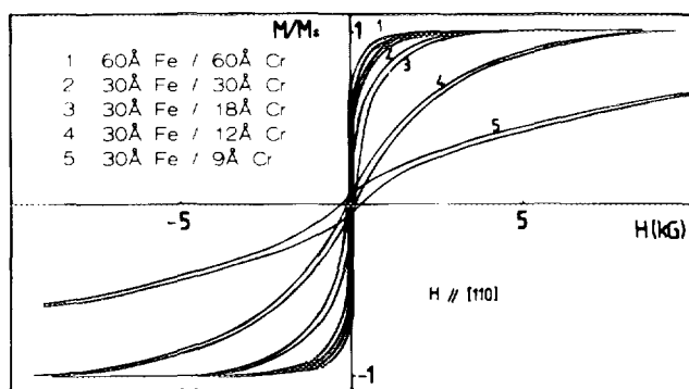
FIG. 1. Magnetization curves at 4.2 K with an applied field along [110] in the layer plane for several Fe(001)/Cr(001) superlattices. The saturation magnetizations M_s are between 1300 and 1700 emu/cm 3 . The measurements presented in this figure have been obtained with a vibrating sample magnetometer and the contribution from the GaAs substrate has been subtracted. Magnetization curves obtained with a SQUID magnetometer have been presented in Ref. 9.
