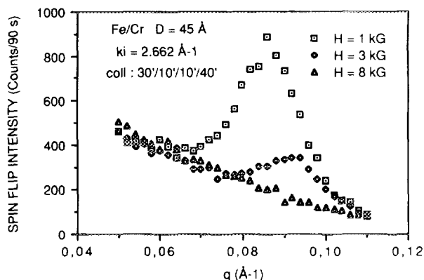
FIG. 4. Field dependence of the spin-flip intensity vs q for a (Fe 30 \text{ \AA}/\text{Cr } 15 \text{ \AA} ) 20 superlattice at 1.6 \text{ K} .
