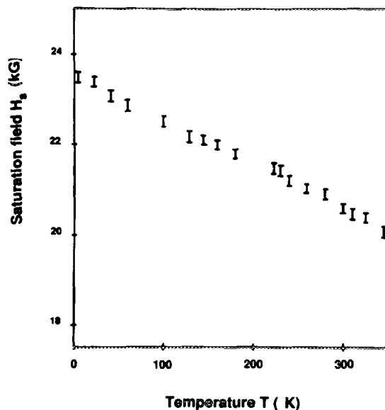
FIG. 3. Temperature dependence of the saturation field H_S for a (Fe 16 \text{ \AA}/\text{Cr } 12 \text{ \AA} ) 20 superlattice.
