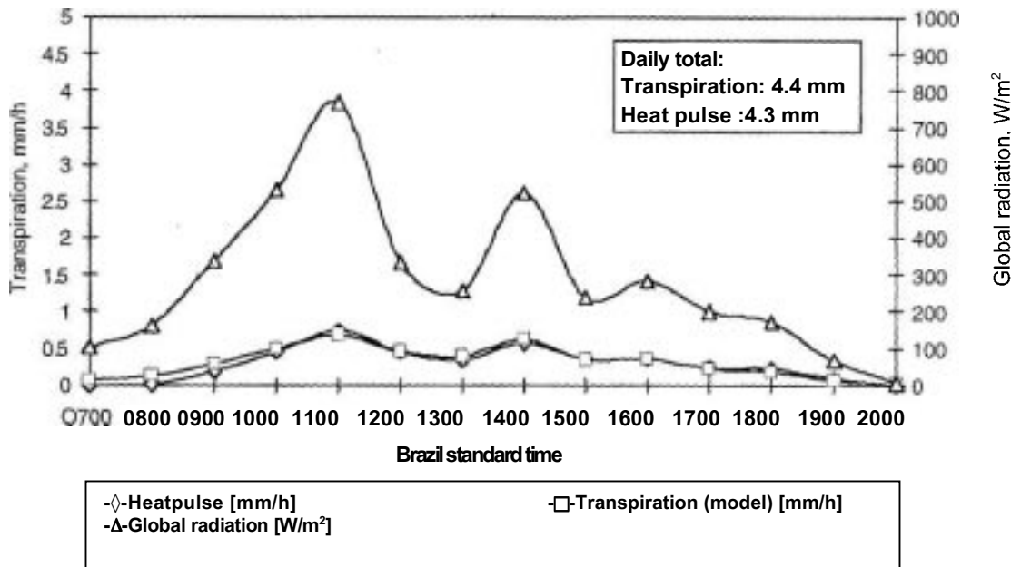
Figure 2. Hourly and daily transpiration estimated by the model and measured by heat pulse technique in maize, with low evaporative demand, on Jan./09/1997.
