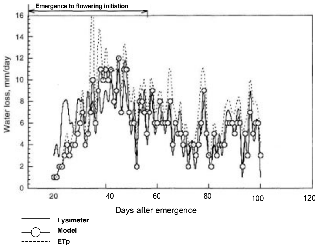
Figure 5. Daily rates of water loss estimated by the model, Penman equation (Etp) and by the lysimeter in maize, during the growing season 1996/1997.
