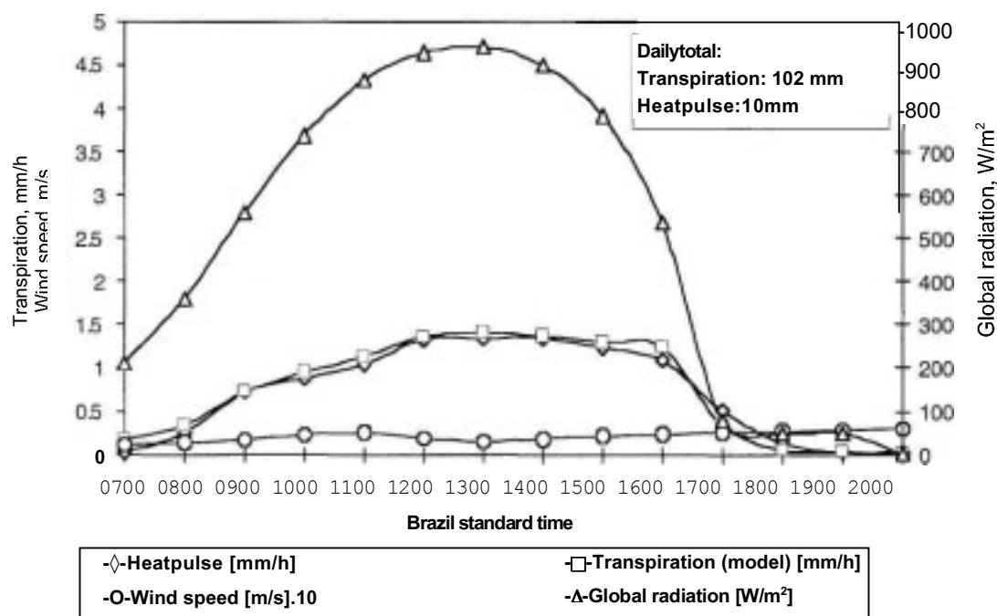
Figure 1. Hourly and daily transpiration estimated by the model and water uptake measured by heat pulse technique in maize, with high evaporative demand, on Dec.17/1995.
