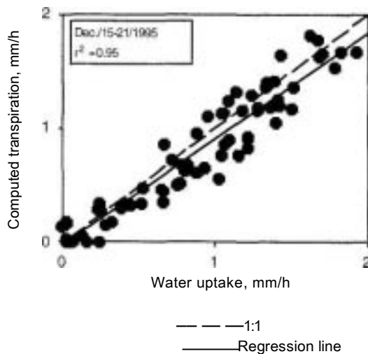
Figure 3. Estimated transpiration vs. measured water uptake by heat pulse technique in maize, during 1995/1996 growing season. Results from regression analysis are shown.
