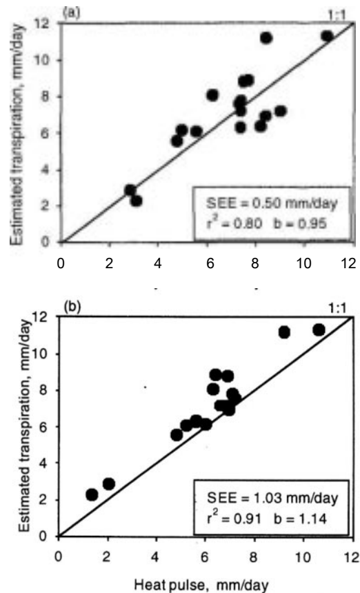
Figure 4. Relationship between estimated transpiration by the model and measured by lysimeter (a) and heat pulse technique (b), during the growing season of 1996/1997. Results from regression analysis and standard error of estimate (SEE) are shown.
