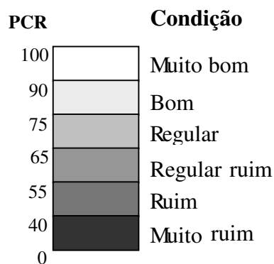
Figura 16. Escala do PCR - Pavement Condition Rating
