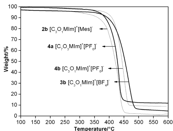
Figure 5. TGA traces of the ILs 2b , 3b , 4a and 4b .
