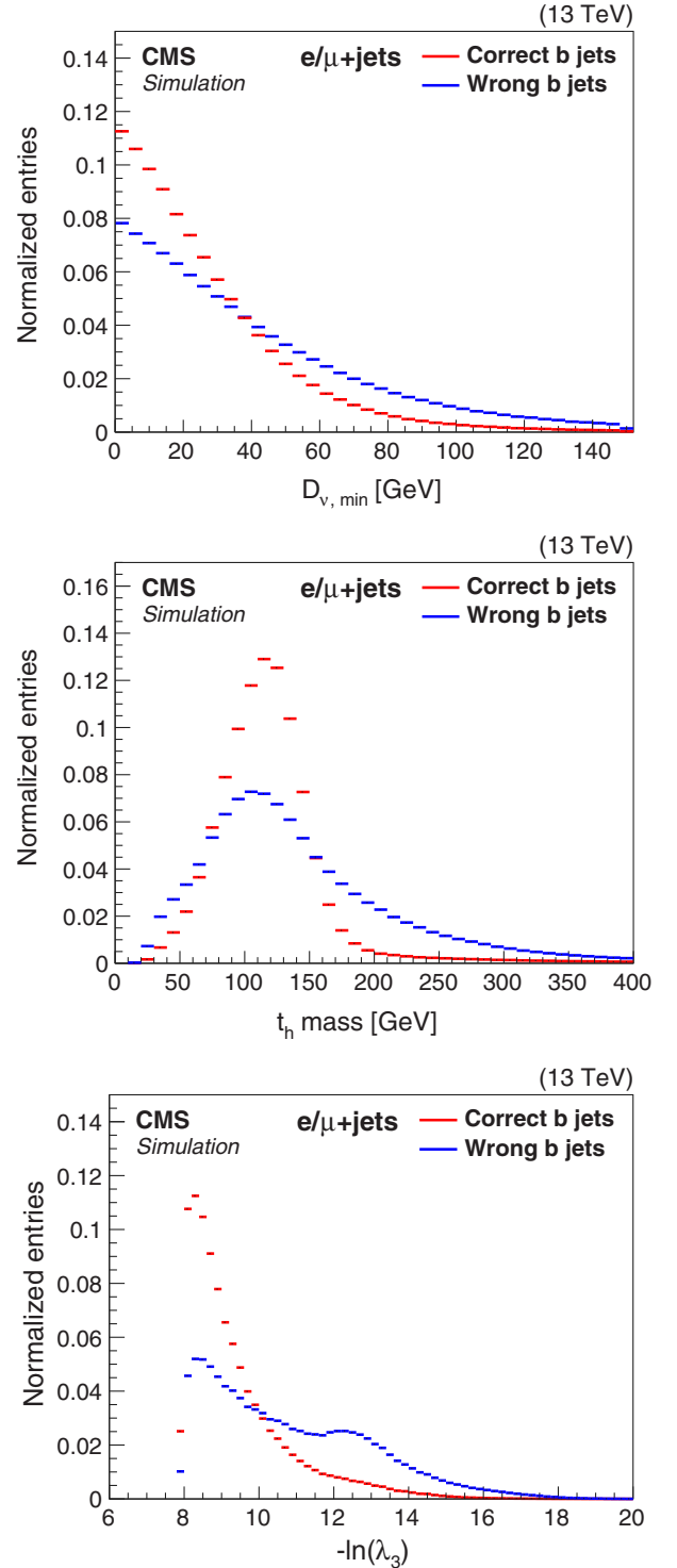
FIG. 3. Three-jet reconstruction. Distributions of the distance D_{\nu,\min} for correctly and wrongly selected b_\ell candidates (top). Mass distribution of the correctly and wrongly selected b_h and the jet from the W boson (middle). Distribution of the negative combined log-likelihood (bottom). All distributions are normalized to have unit area.
