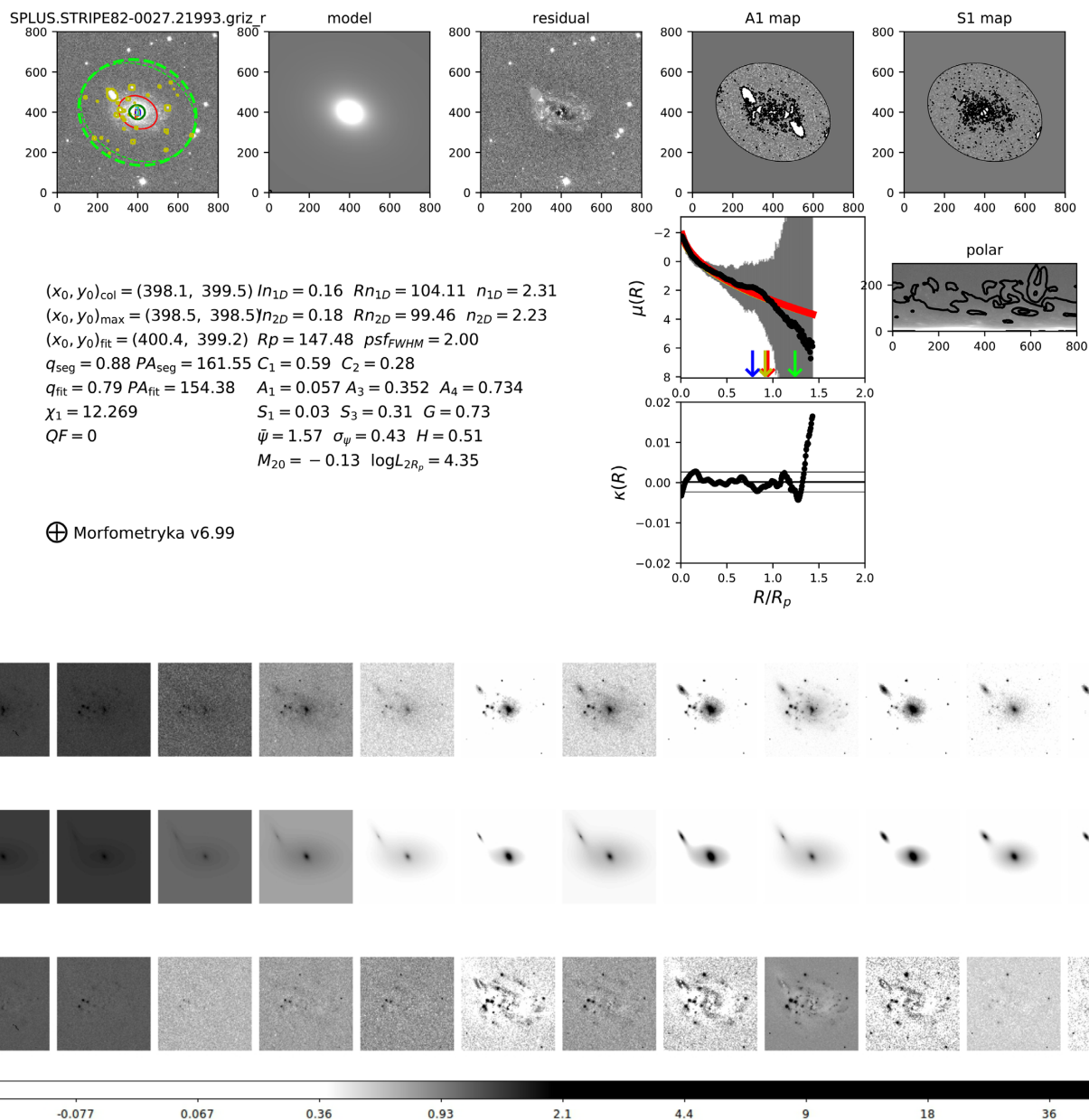
Figure 23. Upper panel: MORFOMETRYKA (top, from left to right): Original image; 2D Sérsic model image; the residual between image and model; asymmetry map used to compute A1; and smoothness map used to compute S1. Bottom: Various measurements (see text for details); Brightness profile (arbitrary units) and model fits; polar map used to compute image gradients and \sigma_{\psi} ; brightness profile curvature. Lower panel: MEGAMORPH-GALFIT: First row – galaxy images in the 12 S-PLUS bands ( u , J0378, J0395, J0410, J0430, g , J0515, r , J0660, i , J0861, and z , respectively); second row – galaxy models as fitted with GALFIT; third row – residuals. The colour bar shows relative intensity measurements with darkest colours indicating largest fluxes.
