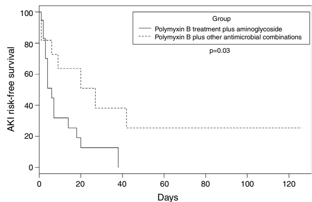
Fig. 1 – Kaplan–Meier curve stratified by polymyxin B plus aminoglycoside treatment and polymyxin B plus other antimicrobial combinations in patients with mediastinitis due to carbapenem-resistant Enterobacteriaceae (CRE).
