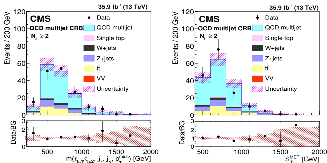
Figure 4. QCD multijet background validation test, using the distributions in CR B m(\tau_{h,1}, \tau_{h,2}, j_1, j_2, p_T^{miss}) (left) and S_T^{MET} (right). The shape of the QCD background is found from data in the loose \tau_h region, CR A and then applied to CR B , defined by p_T^{miss} < 50 GeV and tight \tau_h isolation. For both samples, the non-QCD contributions are estimated from simulation. Note that the normalizations match by construction. The bottom frame shows the ratio between the observed data in CR B and the total background estimation.
