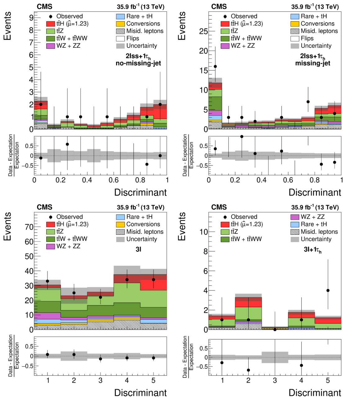
Figure 3. Distributions in the discriminating observables used for the signal extraction in the “no-missing-jet” (top left) and “missing-jet” (top right) subcategories of the 2lss+1\tau_h category, the 3l category (bottom left), and the 3l+1\tau_h category (bottom right), compared to the SM expectation for the t\bar{t}H signal and for background processes. The MEM discriminant LR(2lss+1\tau_h) is used in the 2lss+1\tau_h subcategories, while a D_{MVA} variable, combining the outputs of two BDTs trained to discriminate the t\bar{t}H signal from the t\bar{t}V and t\bar{t}+ jets backgrounds respectively, is used in the 3l and 3l+1\tau_h categories. The distributions expected for signal and background processes are shown for the values of nuisance parameters obtained from the combined ML fit and \mu = \hat{\mu} = 1.23 , corresponding to the best-fit value from the ML fit. The lowest bin of the MEM discriminant in the “missing-jet” subcategory of the 2lss+1\tau_h category collects events for which the kinematics of the reconstructed objects is not compatible with the t\bar{t}H , H \rightarrow \tau\tau signal hypothesis.
