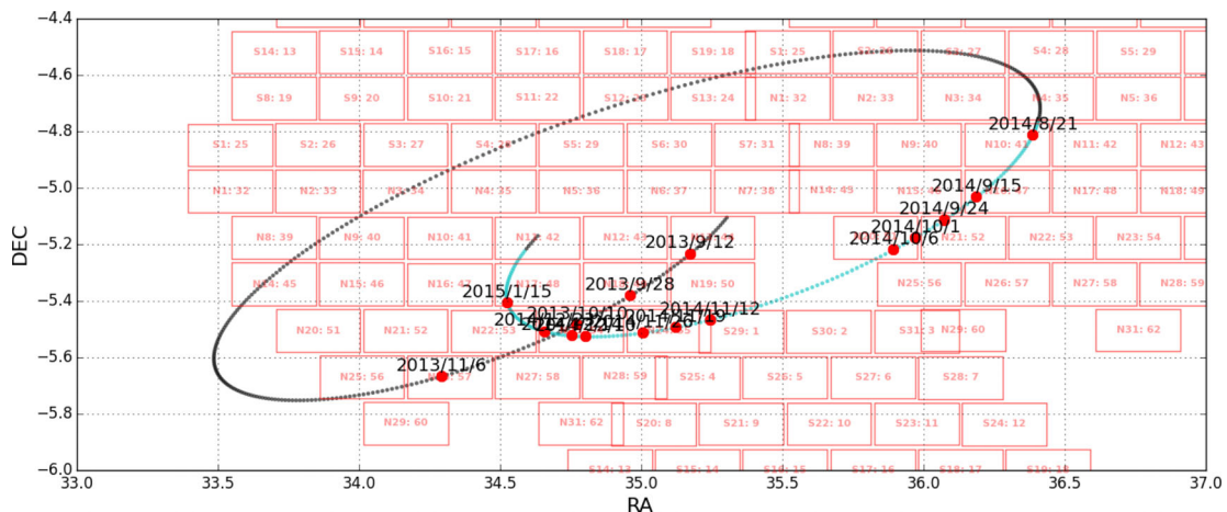
Figure 3. Trajectory of the plutino 2013 RD 98 through three adjacent SN fields during the DES Y1 and Y2 seasons. Large dots indicate nights on which the object was observed by DES. Each rectangle represents one DECcam CCD.
