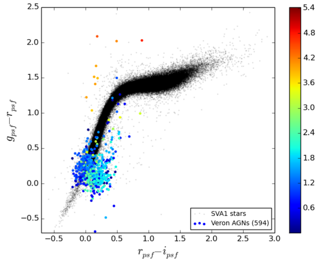
Figure 13. DES gri colour–colour diagram showing the stellar locus as well as known quasars overlapping the DES SV observations. The quasars have been colour-coded according to redshift. While the low-redshift quasars overlap the stellar locus, the z > 4 quasars clearly appear as very red ( g - r ) sources.
