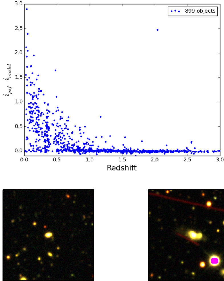
Figure 14. Extended objects can be identified by comparing the PSF magnitude to the model magnitude. Top: the figure shows that many quasars in our sample are resolved (appear to be extended objects) even out to z \sim 1.0 . Bottom: DES gri colour-composite images of two known quasars at z = 0.85 (left) and z = 1.17 (right). Both quasars have extended morphologies in the DES data demonstrating that low surface brightness host galaxy features are clearly visible for quasars out to z \sim 1 .
