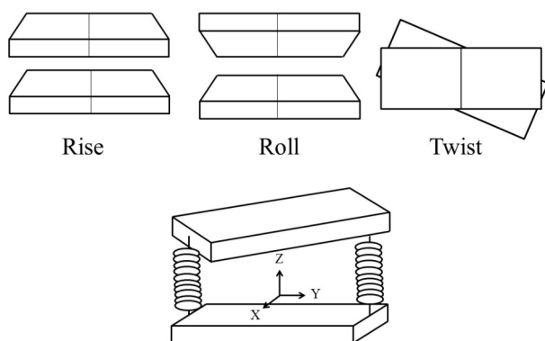
Figure 1. Three selected parameters that describe DNA structure. The base-pairs are shown schematically by solid rectangles linked by springs. 21,22
