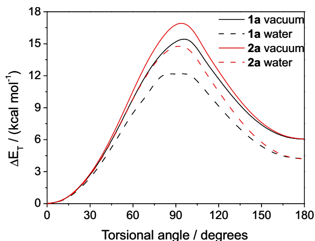
Figure 3. Relative energy ( \text{kcal mol}^{-1} ) \times dihedral angle (degrees) obtained for the ligands 1a and 2a in vacuum and the aqueous medium (DFT/B3LYP with the basis set 6-31G (d)).
