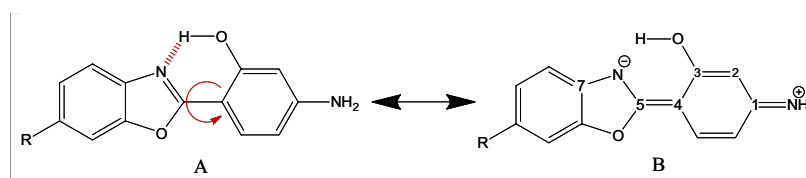
Scheme 1. Schematic representation of the main canonical structures of ligands 2a , 2b and 2c .
