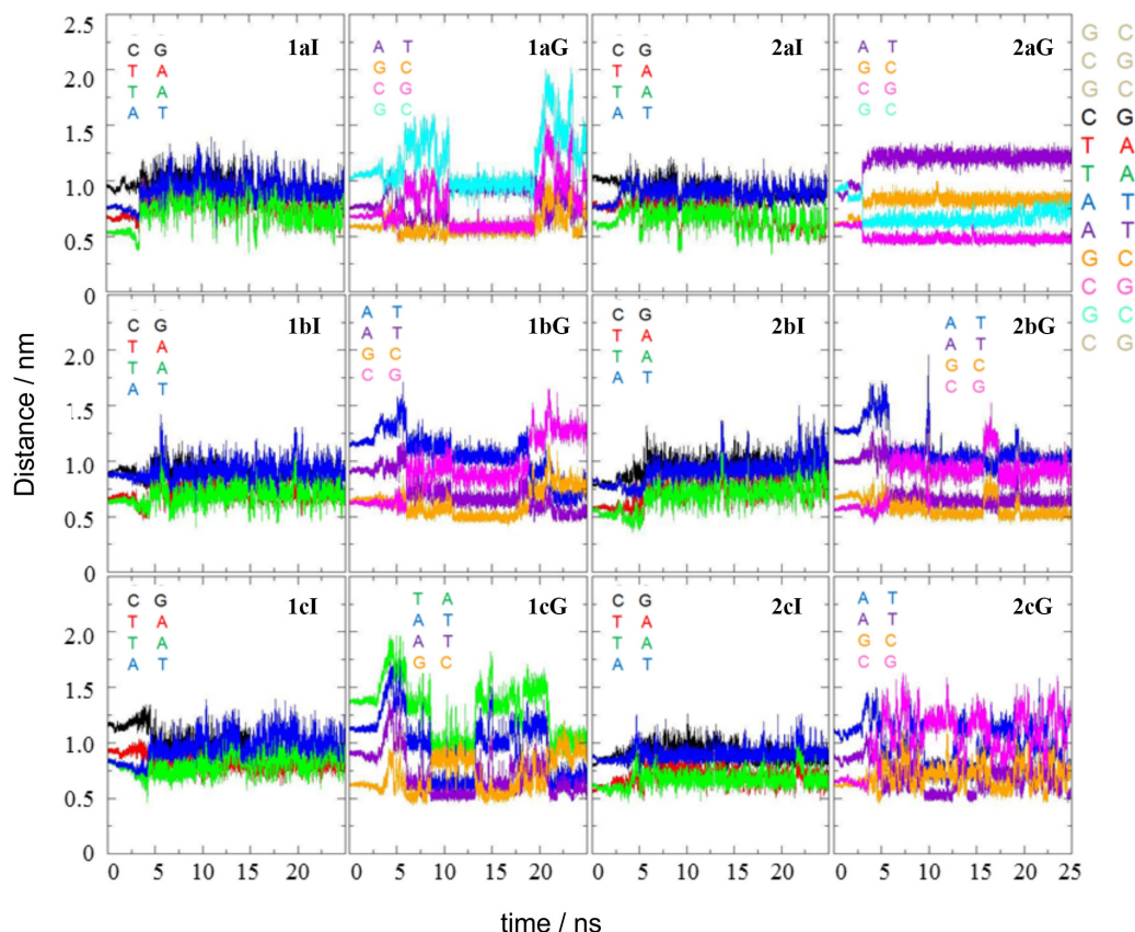
Figure 5. Distance between the center of mass of the ligands and the center of the mass of some base-pairs along the simulations, for all systems. For each system, only the relevant base-pairs were shown. In the upper right corner we show the base-pairs as seen from the minor groove (5' end of the right strand on the top), with the corresponding colors used in the figure.
