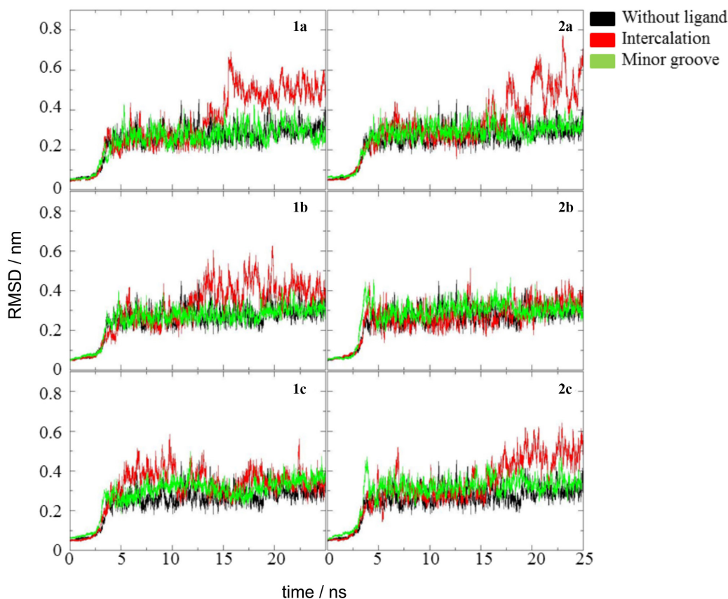
Figure 4. Root mean square deviations (RMSD) of the oligonucleotide. In each case, three simulations were compared: oligonucleotide without ligand, oligonucleotide in presence of an intercalator and oligonucleotide in the presence of a groove binder.
