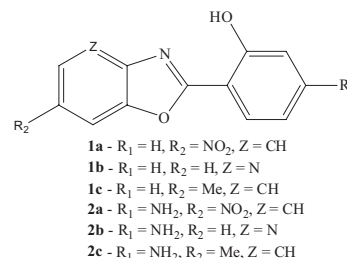
Figure 2. Benzoxazoles derivatives.
