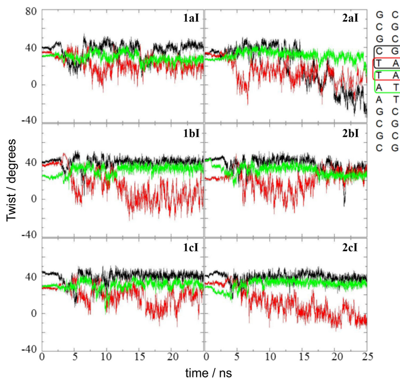
Figure 8. Twist parameter for some relevant base-pair steps for the intercalation binding mode complexes.
