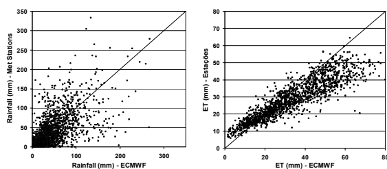
Figure 5. Rainfall and Evapotranspiration (ET) measured (Met Stations) and estimated by ECMWF.
