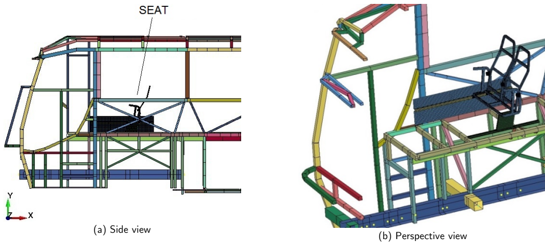
Figure 24 Seat installation.
