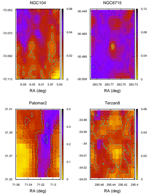
Fig. 2. Differential-reddening maps of NGC 104, NGC 6715, Palomar 2 and Terzan 8. The range of values of \delta E(B - V) is shown by the colour bars.
