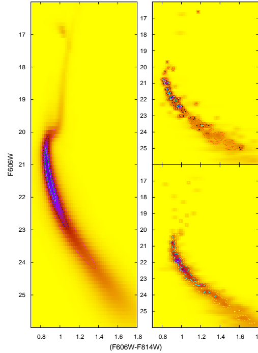
Fig. 1. The bluest (top-right panel) and reddest (bottom-right) Hess diagrams of NGC 6388 are compared to the mean (observed) one (left). The difference in reddening between both amounts to \delta E(B - V) = 0.133 .
