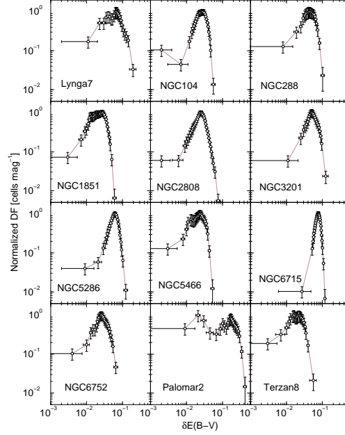
Fig. 3. Distribution function of \delta E(B - V) for a representative GC sub-sample. For comparison purposes, the DFs are normalized by the peak.
