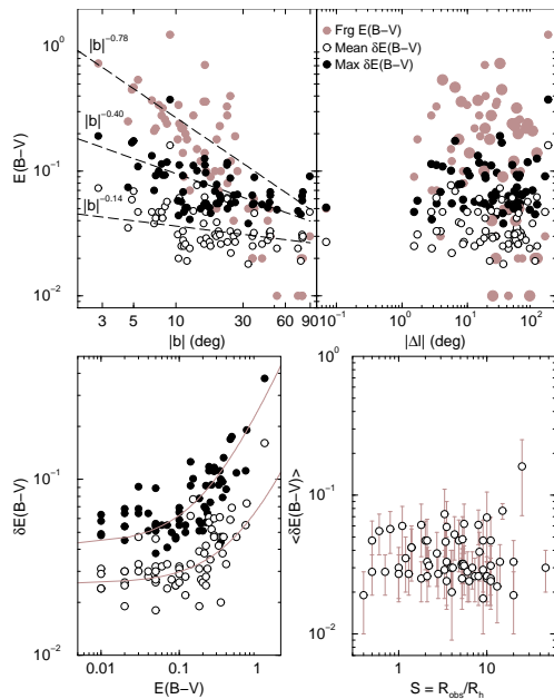
Fig. 4. Reddening parameters as a function of the angular distance to the Galactic plane (top-left), and to the centre (top-right). The dependence on |b| is characterized by power-laws (dashed lines). \delta E(B-V)_{max} and \langle \delta E(B-V) \rangle are mildly correlated with E(B-V) (bottom-left). There is no correlation between \langle \delta E(B-V) \rangle and the GC area covered by WFC/ACS (bottom-right).
