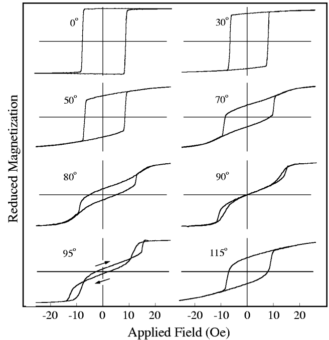
FIG. 2. Experimental in-plane hysteresis loops for several angles (from 0° to 120°) between the field and the easy axis.
