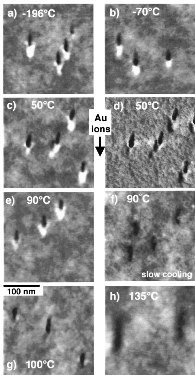
FIG. 2. TM-SFM images of PMMA targets bombarded by 20 MeV Au ions at temperatures between -196 and 135 °C. Targets were water-cooled immediately after the \approx 3 s irradiation time, except on (f) where a slow cooling rate was used. Note the remarkable change in the rate of relaxation of the hillocks between (e) 90 °C and (g) 100 °C. (d) shows the phase image corresponding to the height image given in (c). The contrast covers height variations in the 8 nm range in (a)–(c), (e)–(h) and phase angle variations in the 30^\circ range in (d). The impact angle is 79^\circ to the surface normal. The arrow indicates the ion penetration direction and the slow scanning axis of the microscope.
