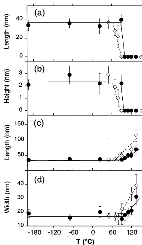
FIG. 3. Average dimensions of surface features induced by 20 MeV Au ions impacting PMMA thin films as a function of target temperature and cooling rate: (a) hillock length, (b) hillock height, (c) crater length, (d) crater width. Slow cooling data are depicted as open diamonds and fast cooling data as circles. The solid and dashed lines are just to indicate the trend of the two relaxation conditions. Mean values were obtained from data collected from around 100 impact sites for each temperature, using different SFM tips.
